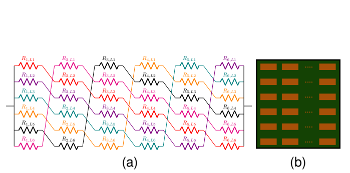
Fig. 7. Transposing the coil geometry across layers as shown in (a) ensures a balanced induced back-emf between layers of planar conductor (b).
