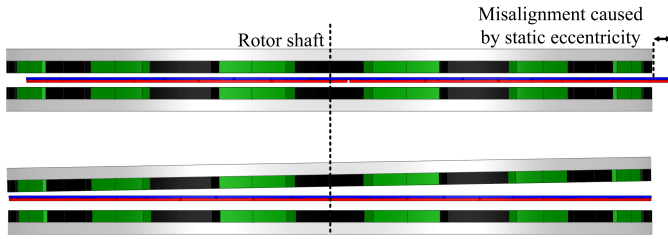
Fig. 4. Two rotor asymmetry conditions. Uneven airgap or tolerances in magnet remanences and static eccentricity.
