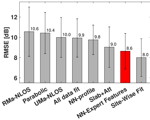
Fig. 10: Model Selection RMSE results. The error bars indicate \pm one standard deviation of the testing RMSE across different sites.
