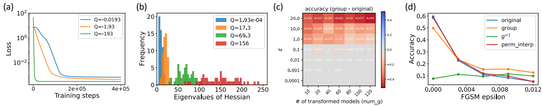
Figure 2: Overview of empirical observations with more details in Appendix G, H, and I. (a) In a two-layer neural network, the convergence rate depends on the conserved quantity Q . (b) The distribution of the eigenvalues of the Hessian at the minimum is related to the value of Q . (c) The ensemble created by group actions has similar loss values when \varepsilon is small. (d) The ensemble model improves robustness against fast gradient sign method attacks.
