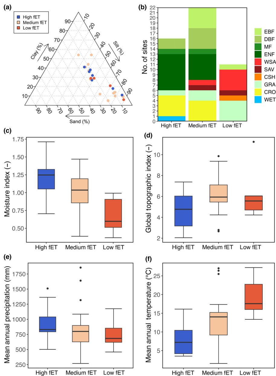
Fig. 7 Analysis of soil and climate variables per group of fractional reduction in evapotranspiration (fET) group, see the Site selection and binning section). (a) Triangular plot of soil texture, colored by site, plotted with R package 'PLOTrix' (Lemon, 2006). Note that some sites are overlapping. (b) IGBP vegetation classes (CRO, cropland; CSH, closed shrubland; DBF, deciduous broadleaf forest; EBF, evergreen broadleaf forest; ENF, evergreen needleleaf forest; GRA, grasslands; MF, mixed forest; SAV, savannah; WET, wetland; WSA, woody savannah). (c) Moisture index, defined as the ratio of annual precipitation (P) over potential evapotranspiration (PET), calculated for all available years on a site-by-site basis. Precipitation data was taken from the FLUXNET2015 dataset, whereas PET was calculated with the SPLASH model, based on a Priestley–Taylor formulation of evapotranspiration. (d) Global topographic index (GTI), defining the tendency of the soil to become saturated with water because of its topographic position. Higher GTI values are typical in valleys, whereas lower values are most common at ridgetops. (e) Mean annual precipitation (MAP). (f) Mean annual temperature (MAT). The bold black lines in the boxplots represent the median. The lower and upper hinges correspond to the first and third quartiles. Data beyond the hinges are plotted individually.
