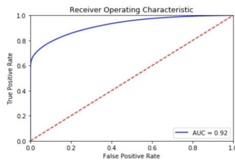
Figure 9: ROC-AUC curve of decision tree.
