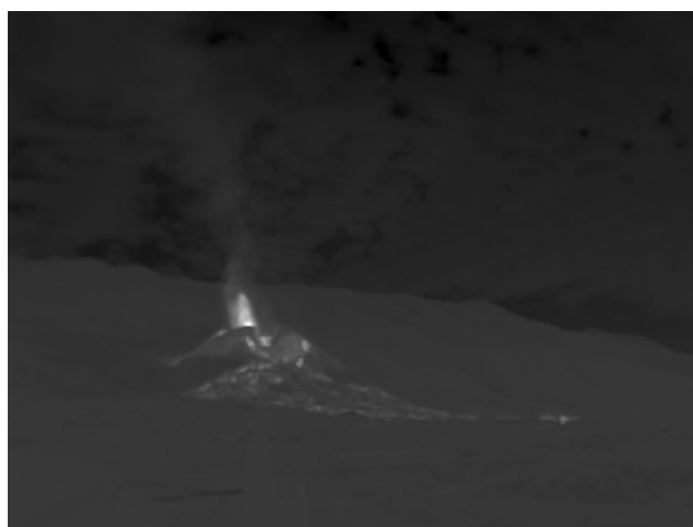
Figure 8: Thermal infrared images of the main vent at the 2021 Cumbre Vieja eruption, which were provided to the exercise participants as simulated footage from the scenario vent during Stage 3 of the activity. Participants were able to extract time series of plume height from the provided footage. Source: LDEO / AVERT camera system. Full image catalog can be found in http://vulcan1.ldeo.columbia.edu/vulcand/ldeo/raw/data/siteCv/ .
