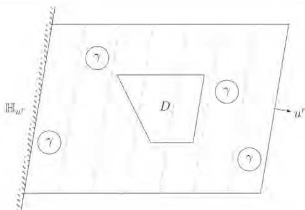
FIGURE 6 A u^r -crossed u^r -strip S together with a possible (u^r, \gamma) -partition for S \cap A in which a_1 = a_2 = a_4 = a_5 = 1 and a_3 = 3
