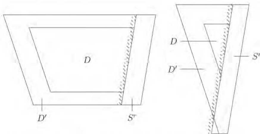
FIGURE 9 Two possible configurations of the droplets in Lemma 8.28. The hatching indicates the sites that would be assumed to be present for the purposes of the event that S^r is u^r -crossed. In the first example, the event \Delta(D, D') implies that S^r is u^r -crossed, but in the second it does not, for example, if A \cap D' is the set of dots in S^r
