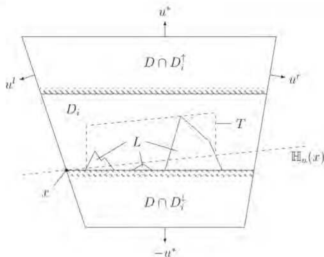
FIGURE 8 The figure depicts the application of Lemma 8.26 in the proof of Lemma 8.25 assuming \alpha^-(u^*) = \infty . T is the minimal u -strip such that L \subset T \cup \mathbb{H}_u(x) , where \sigma(u) = p^{1-\eta} , and is u -crossed by A .
