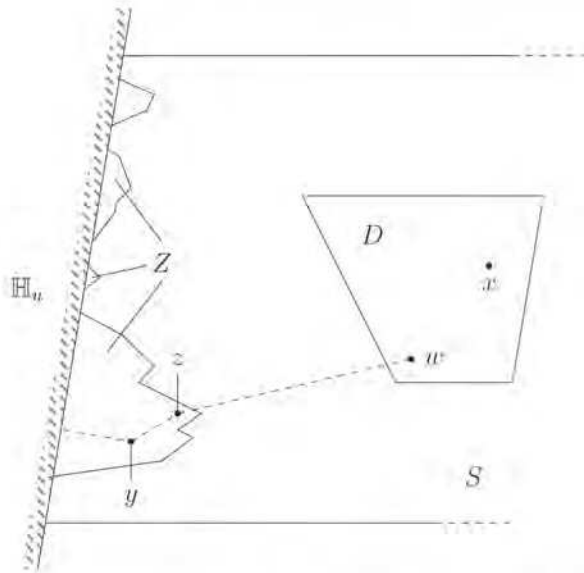
FIGURE 7 The situation in the proof of Claim 8.22 is depicted assuming z \in Z . The size of the projection |\langle D - \mathbb{H}_u, u \rangle| is at most the total length of the dashed line in the u -norm.
