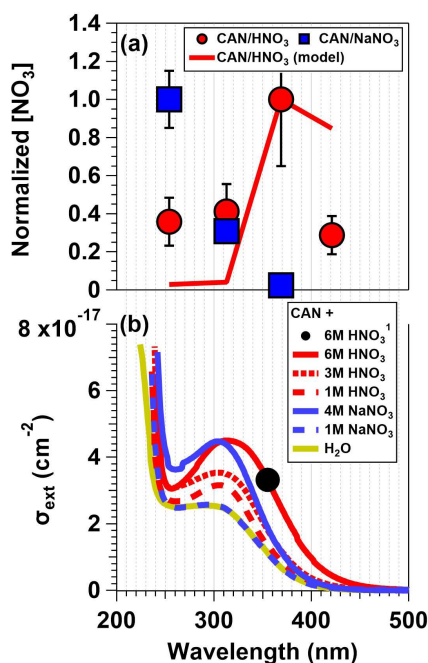
Figure 3. (a) [\text{NO}_3] values obtained from irradiated CAN and 6.0 M \text{HNO}_3 and CAN and 4.8 M \text{NaNO}_3 mixtures as a function of irradiation wavelengths. Results were normalized to [\text{NO}_3] achieved with irradiation of CAN/ \text{HNO}_3 mixtures at \lambda = 369 \text{ nm} or CAN/ \text{NaNO}_3 mixtures at \lambda = 254 \text{ nm} . Error bars represent \pm 1\sigma uncertainty in binned [\text{NO}_3] values. (b) Extinction cross sections ( \sigma_{\text{ext}} ) of CAN/ \text{HNO}_3 and CAN/ \text{NaNO}_3 mixtures (for details see Sect. 2.3). The black dot (note the superscripted 1 in the legend) corresponds to data from Wine et al. (1988).
