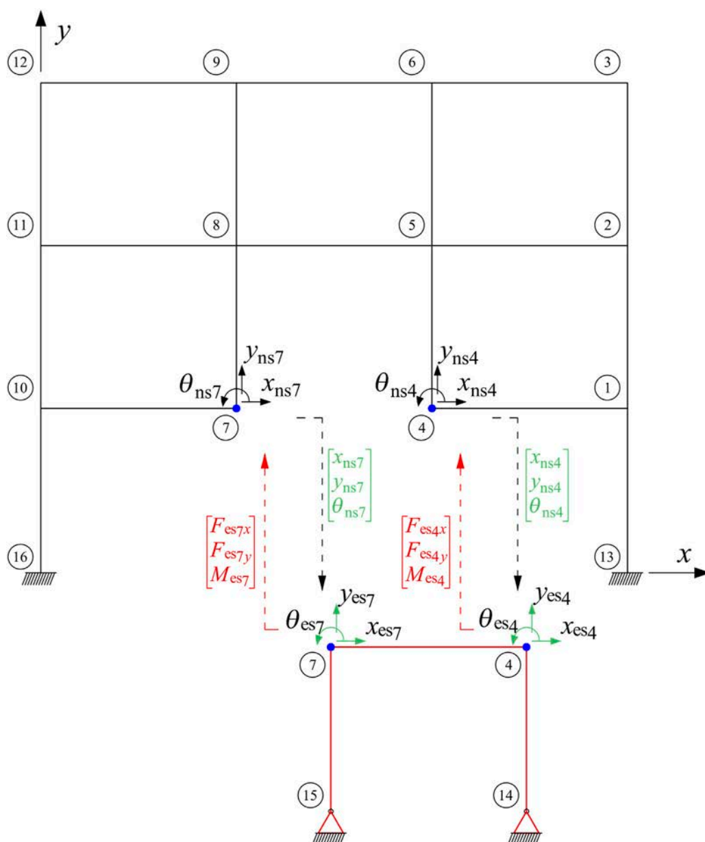
FIGURE 5 Partitioned system in closed loop.
