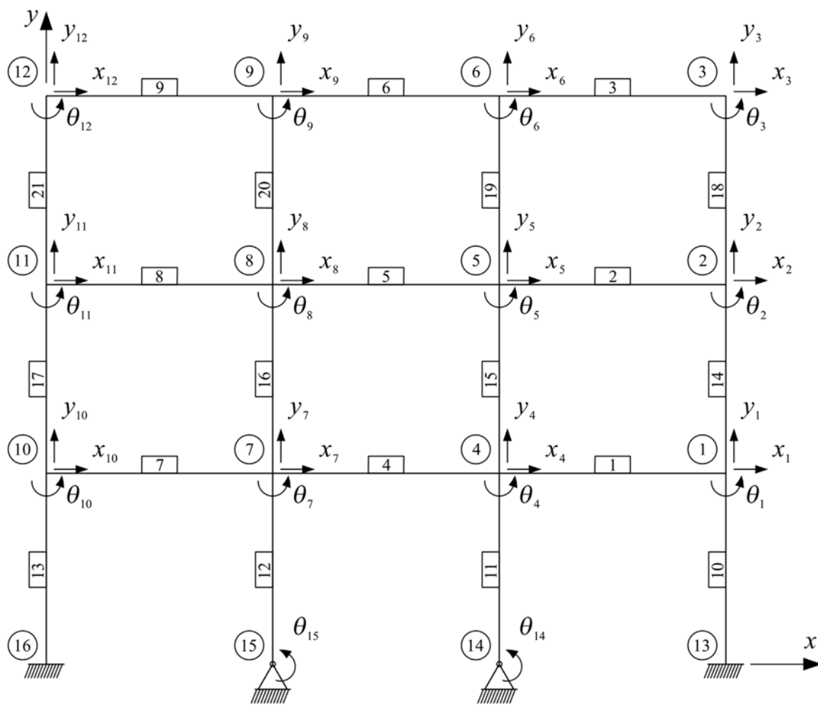
FIGURE 2 FE model description.
