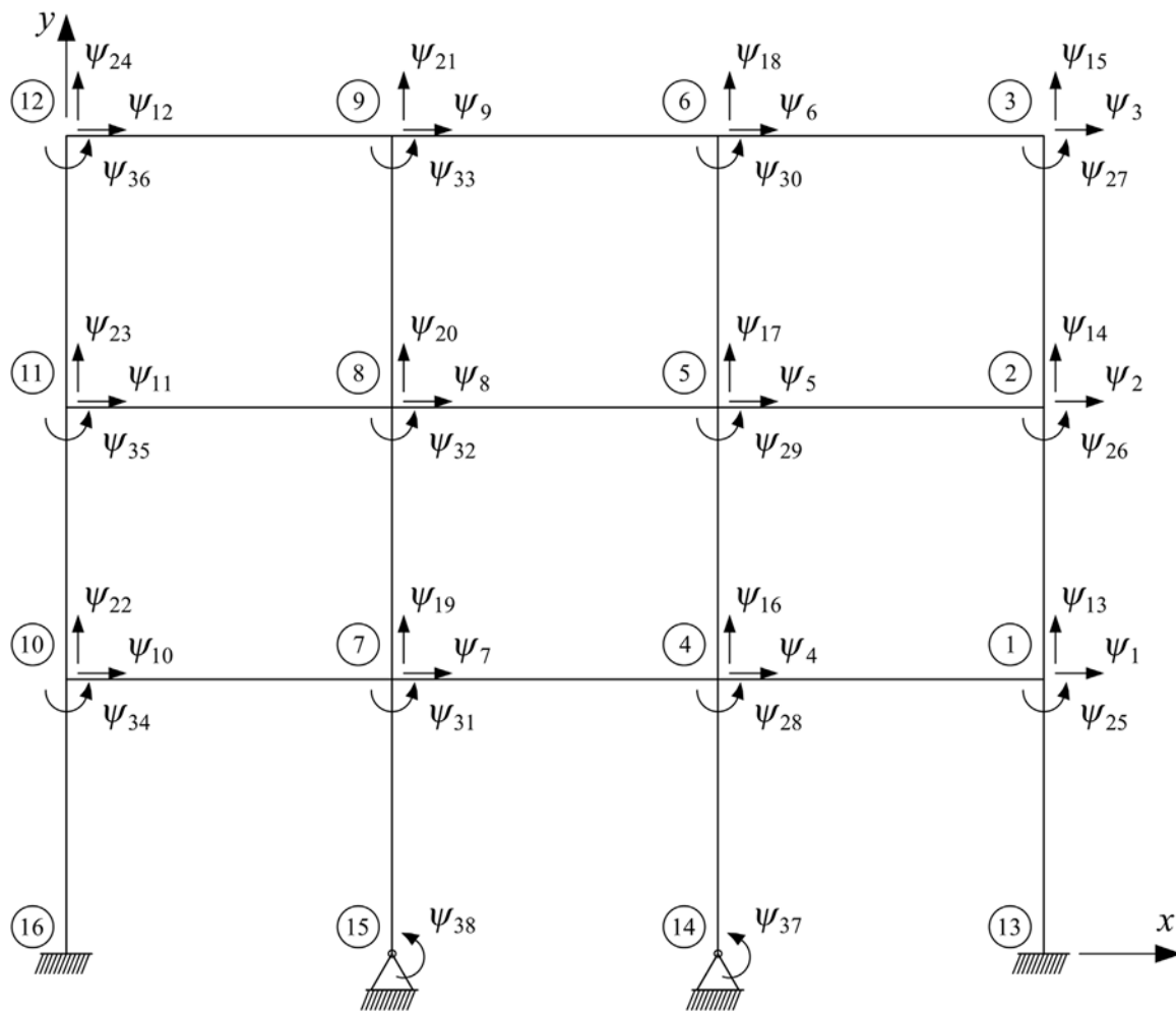
FIGURE 3 Definition of the DOF vector in Eq. 2.
