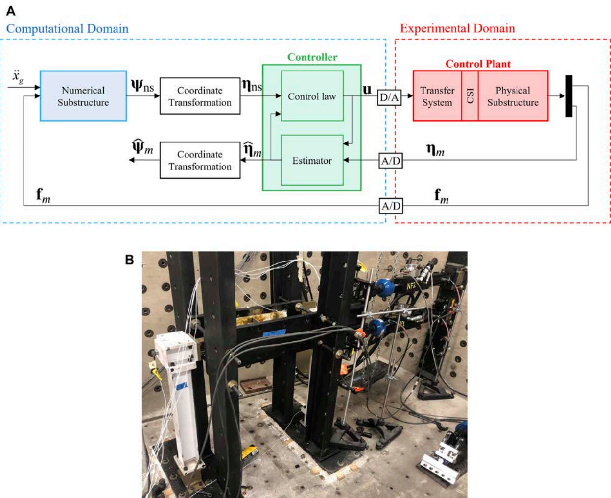
FIGURE 13 maRTHS scheme and control plant implementation in the IISL laboratory. (A) Block diagram of the maRTHS, (B) The control plant.
