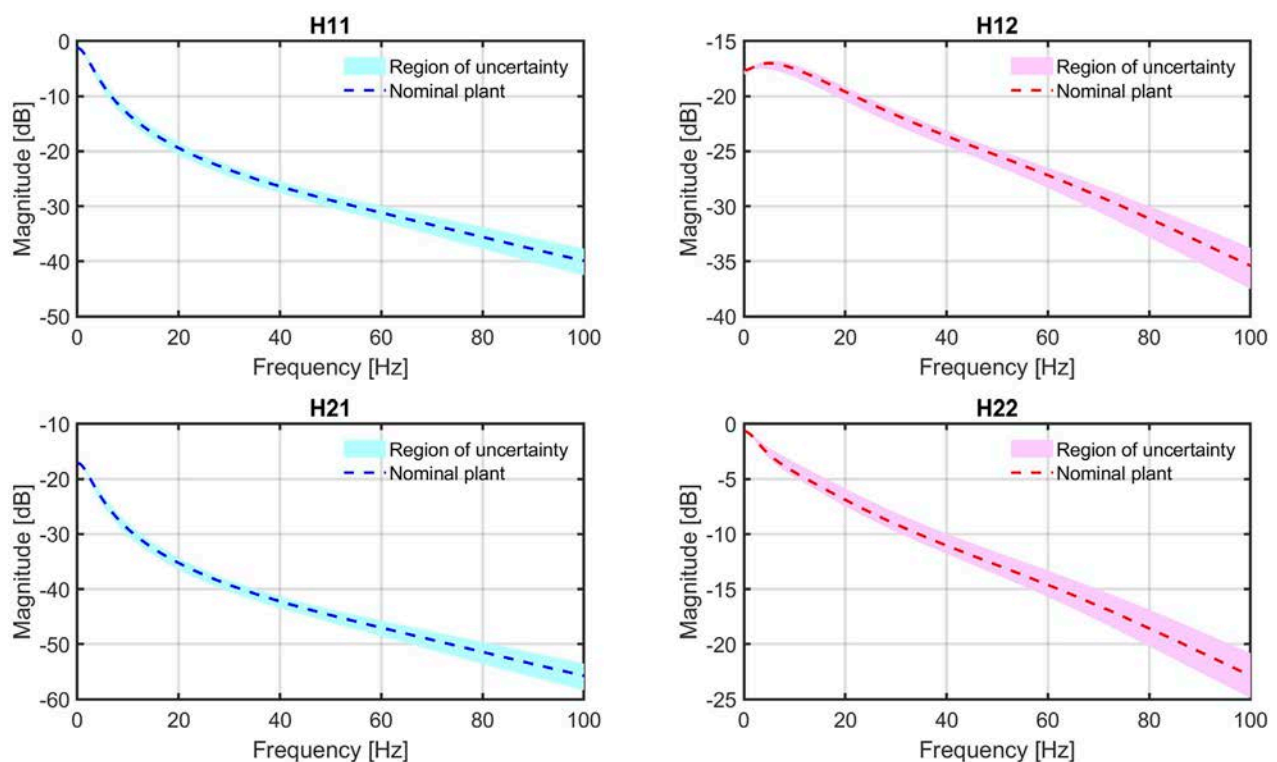
FIGURE 20 FRF regions for the plant model uncertainty.
