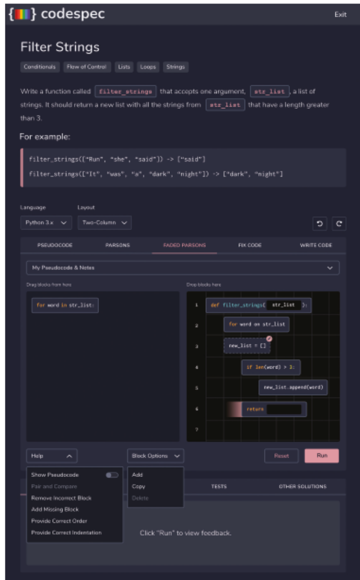
Figure 1: codespec filterStrings
