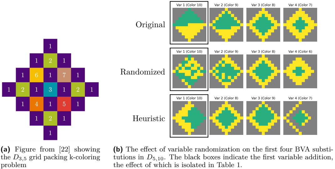
Figure 3 The auxiliary variables introduced by BVA on the packing k -coloring problem are sensitive to randomization.
