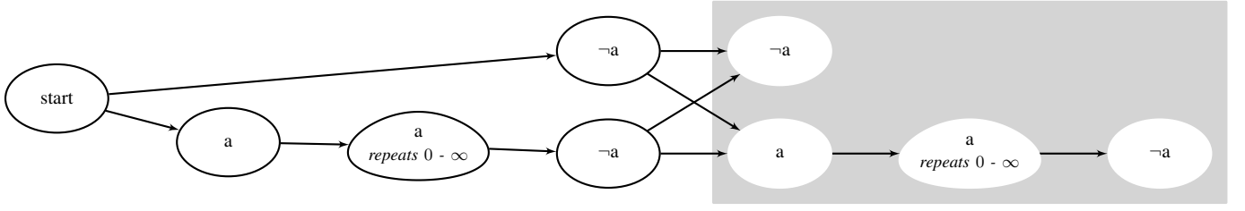
Fig. 4: Timeline visualization for \omega -regular expression ((\neg a)|(aa^*(\neg a))((\neg a)|(aa^*(\neg a)))^\omega .
