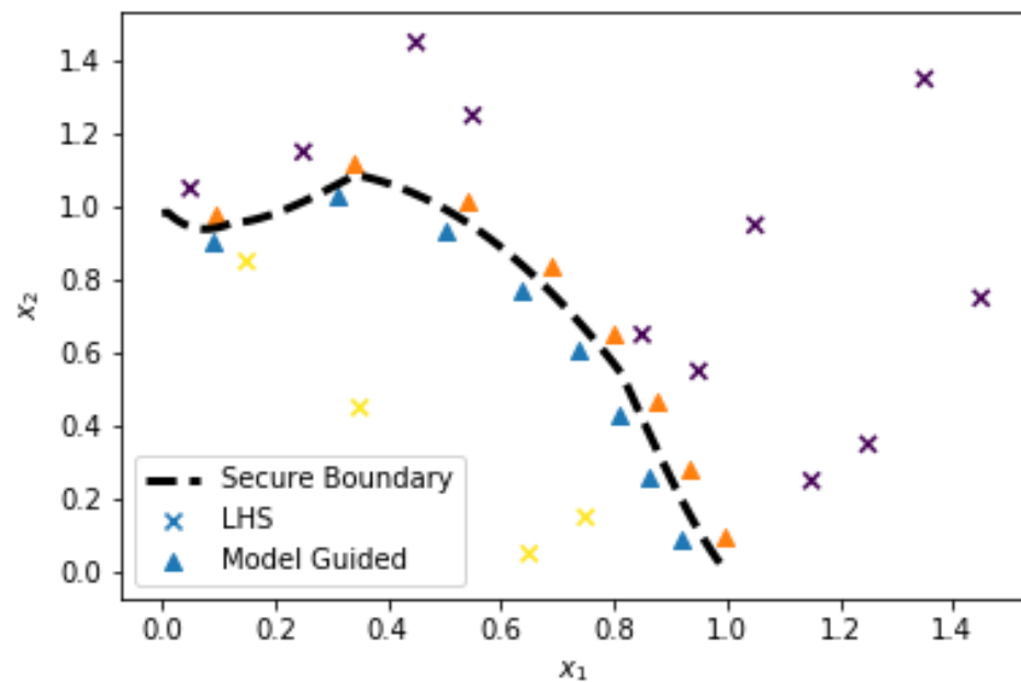
Figure 4. Illustration of Points from Model Guided Sampling and from Space-filling Approach. Color definitions: purple 'x' points are infeasible LHS points, orange triangles are infeasible model-guided samples, blue triangles are feasible model-guided samples and yellow 'x' points are feasible LHS samples (LHS).
