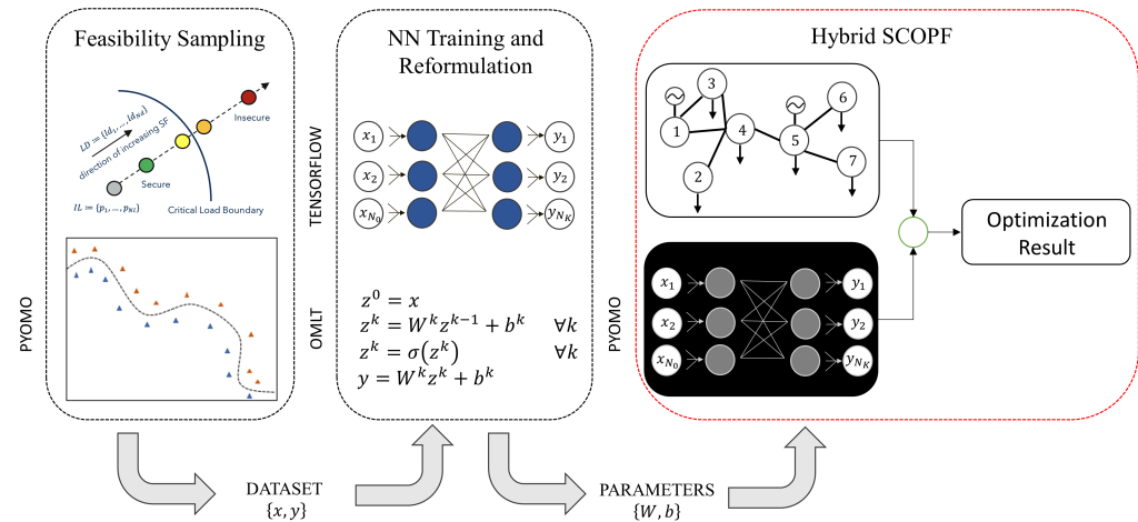
Figure 1. Summary of Key Methodologies and Novel Contributions in this Work. Sampling, NN Training and Reformulation, and Hybrid Solution are explained in full detail in Sections 4–6 respectively. (Dotted black outline covers offline processes, while dotted red-line covers online processes).
