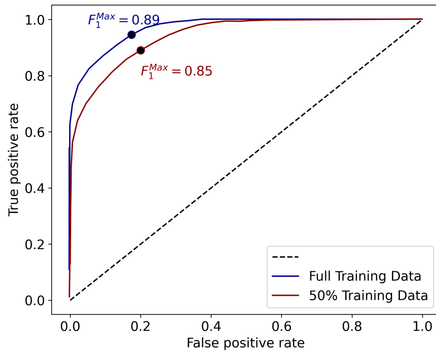
Figure 6. Receiver Operating Characteristic (ROC) Curve for Security Predictions (Case 118, 6 cont.). Comparison Shows the effect of Training Data on Classifier Performance.
