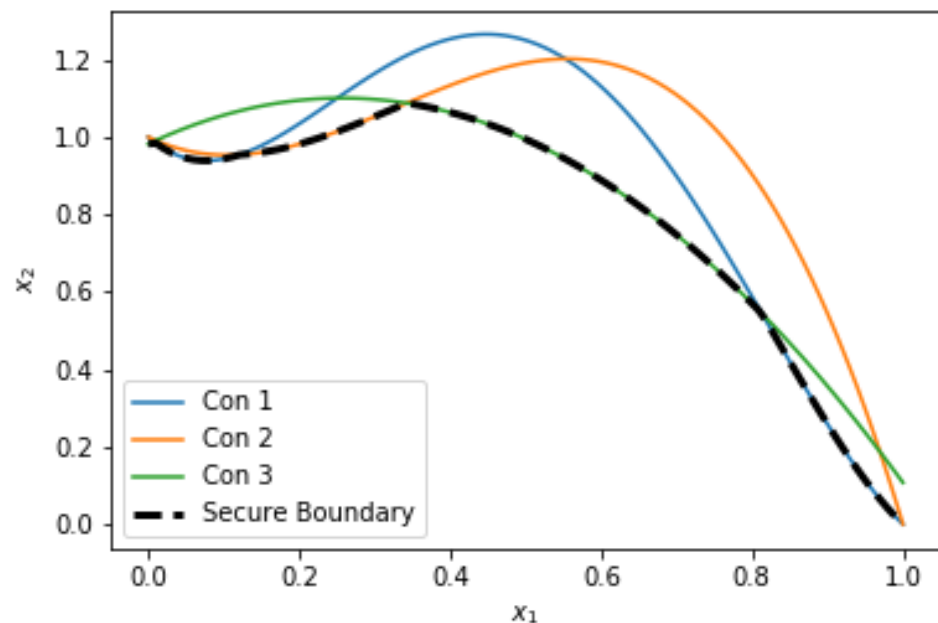
Figure 3. Secure Space of Multiple Non-Convex Constraints.
