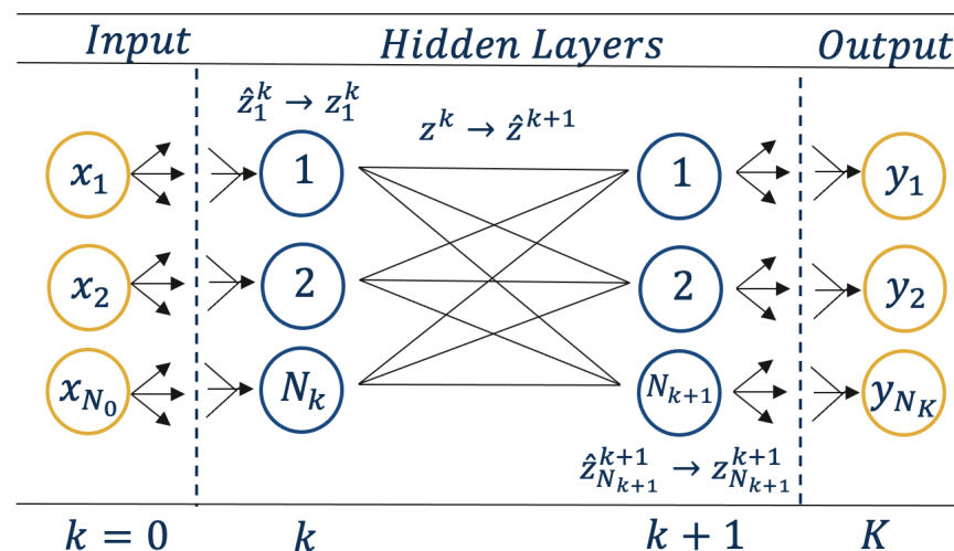
Figure 5. Depiction of Neural Network Architecture.
