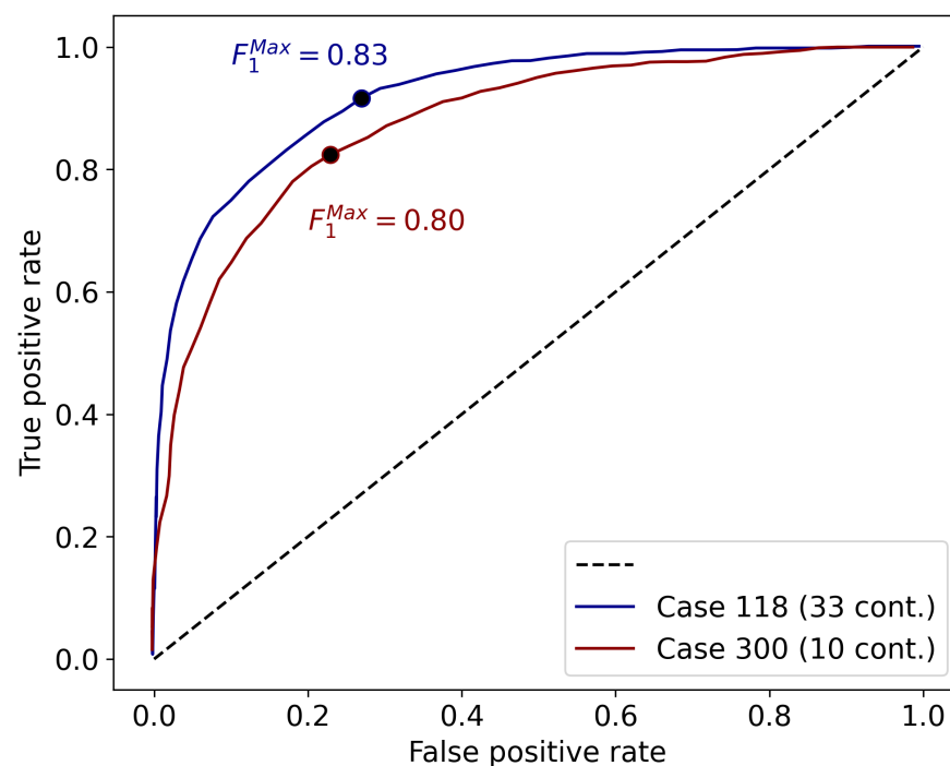
Figure 7. Receiver Operating Characteristic (ROC) Curve for Security Predictions on Test Data for Case 118, 33 cont. and Case 300, 10 cont. Comparison Shows the Effect of Scaling Up the Problem Dimension with Respect to Contingency and Number of Buses
