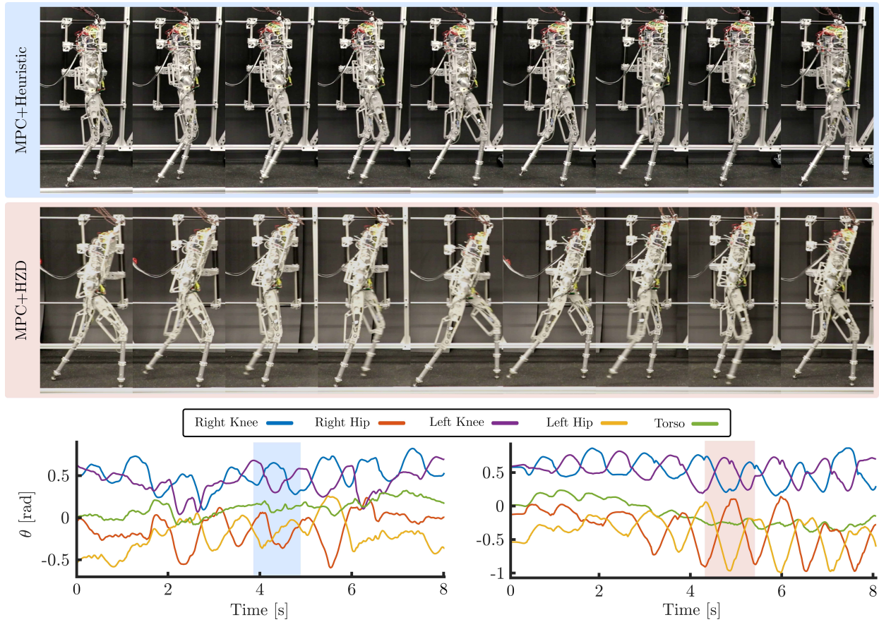
Fig. 6: Gait tiles and joint angle trajectories for forward walking behavior of the whole body MPC at a horizon length of 1 second (top, left), and the whole body MPC+HZD at a horizon length of 0.5 seconds (bottom, right). The HZD reference induces stronger periodic behaviors in the joint coordinates, correlated with the periodic nature of an HZD gait.
