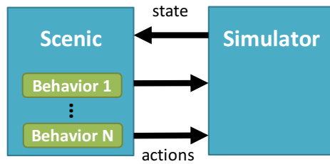
Fig. 8: Diagram showing interaction between SCENIC and a simulator during the execution of a dynamic scenario.
