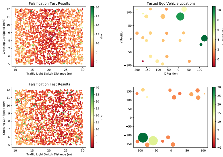
Fig. 12: Falsification results in CARLA. Top: Town05; bottom: Town03.
