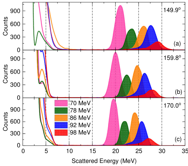
Fig. 1. Typical energy spectra of backward angle scattering at three laboratory angles and five typical beam energies. The filled curves in each panel beyond 15 MeV scattered energy, represent the QEL events. The events below 10 MeV are mostly due to the evaporated Light Charged Particles (LCPs).
