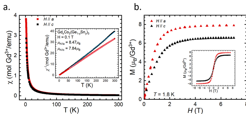
Figure 6. Anisotropic magnetic measurements of \text{Gd}_x\text{Co}_3(\text{Ge}_{1-y}\text{Sn}_y)_3 . (a) Temperature-dependent magnetic susceptibility, \chi(T) , collected for temperature T = 1.8 –300 K. (Inset) The Curie–Weiss fits were applied to inverse susceptibility, \chi^{-1} , as described in the text and are represented by solid lines. (b) Anisotropic field-dependent magnetization, M(H) , collected at T = 1.8 K and for -7 < H < 7 T.
