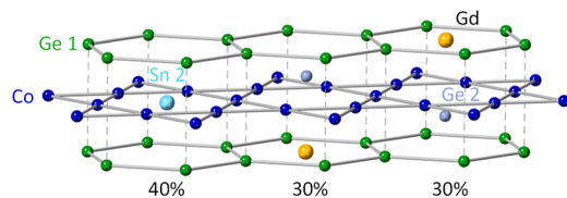
Figure 3. \text{Gd}_x\text{Co}_3(\text{Ge}_{1-y}\text{Sn}_y)_3 ( x = 0.3 , y = 0.133 ) structure is expanded to show the three random possible configurations of the disordered model. The percent occupancy of each configuration is provided. The dashed lines from Ge1–Ge1 are meant to guide the eye. Bonding between the Ge honeycomb nets and the Co kagome nets has been selectively omitted.
