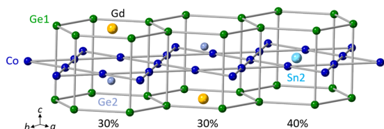
Figure 2. Crystal structure of \text{Gd}_x\text{Co}_3(\text{Ge}_{1-y}\text{Sn}_y)_3 and site symmetry of each atomic position.
