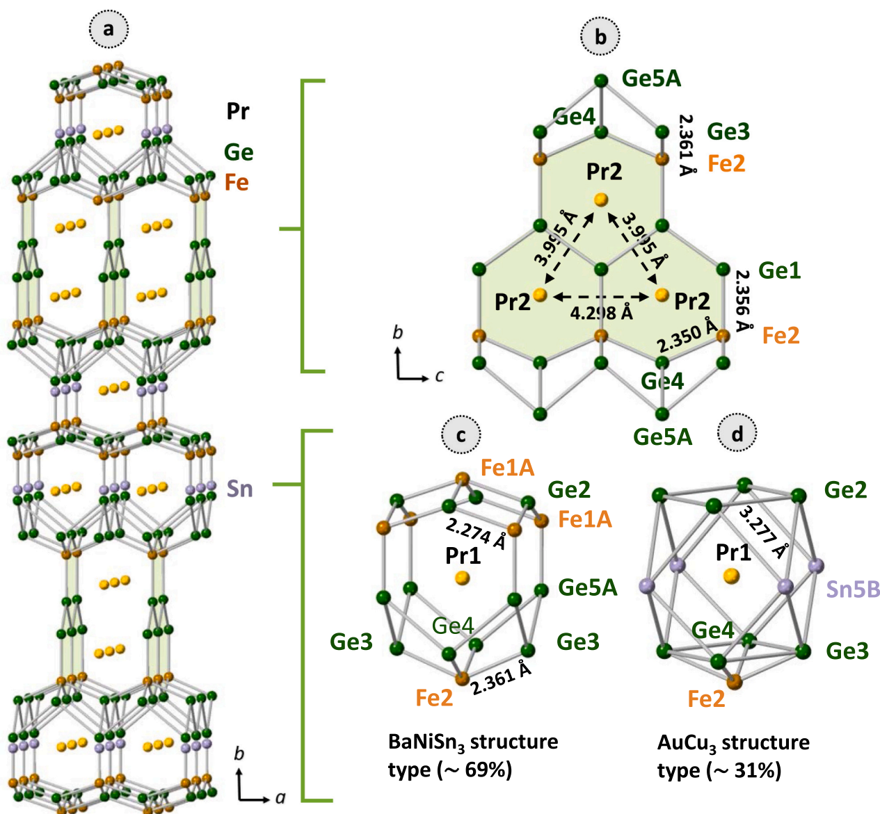
Fig. 4. The atoms, Pr, Fe, Ge, and Sn are shown as yellow, dark orange, green, and purple, respectively. The structure of \text{Pr}_4\text{Fe}_3\text{Ge}_{10} is viewed along the c -axis (a). The \text{CeNiSi}_2 subunit contains Pr2 atomic sites as shown in (b) with the \text{ThSi}_2 structure type highlighted in green. The disorder model for \text{Pr}_4\text{Fe}_3\text{Ge}_{10} is shown for the Pr1 local environment and can be broken down into two partially occupied structure types: \text{BaNiSn}_3 (c) and \text{AuCu}_3 (d), with the percent occupancy specified.
