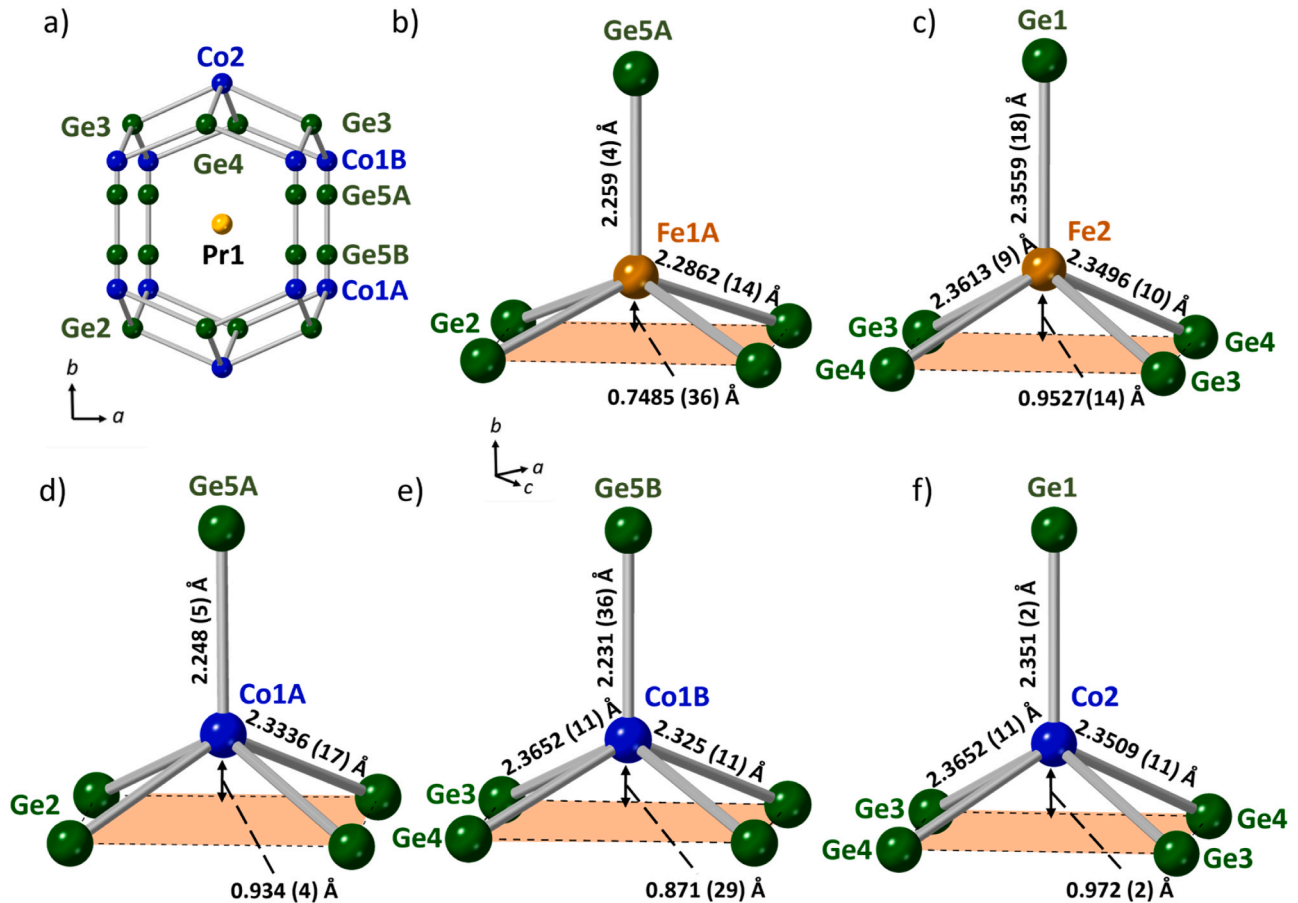
Fig. 9. (a) The disorder of the \text{BaNiSn}_3 subunit in \text{Pr}_4\text{Co}_3\text{Ge}_{10} is shown with the typical orientation marked as Co1A-Ge5A and the inverted orientation as Co1B-Ge5B. The (b) Fe1A, (c) Fe2, (d) Co1A, (e) Co1B, and (f) Co2 sites are compared for \text{Pr}_4\text{Fe}_3\text{Ge}_{10} and \text{Pr}_4\text{Co}_3\text{Ge}_{10} . The transition metal-Ge distances and distance from the basal Ge plane (highlighted in orange) are given.
