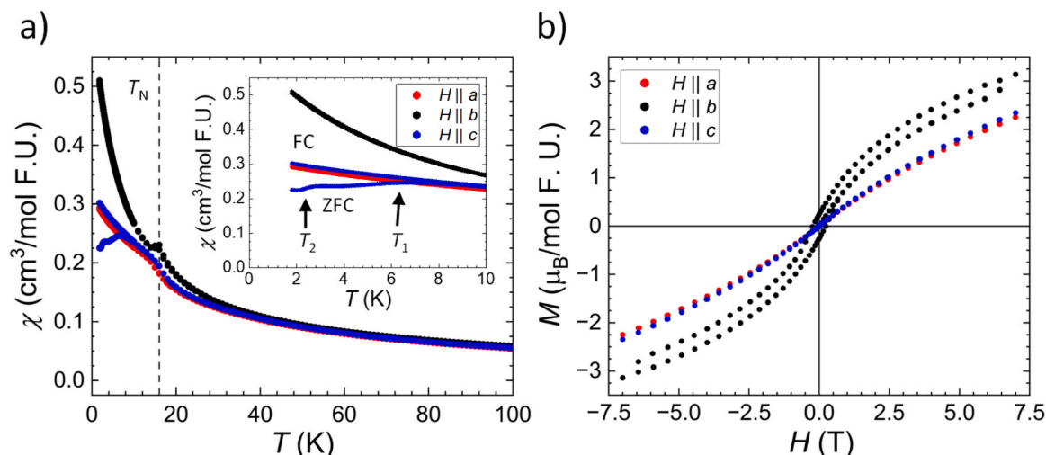
Fig. 7. (a) The magnetic susceptibility (at 0.1 T) as a function of temperature is shown for \text{Pr}_4\text{Co}_3\text{Ge}_{10} . (b) Magnetization as a function of magnetic field at 1.8 K is shown for \text{Pr}_4\text{Co}_3\text{Ge}_{10} . H//a , H//b , and H//c are shown as red, black, and blue, respectively.
