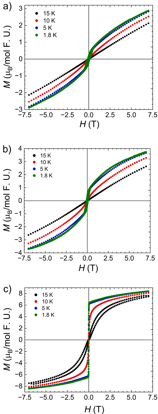
Fig. 6. Magnetization as a function of magnetic field is shown for \text{Pr}_4\text{Fe}_3\text{Ge}_{10} (a) along the a -direction ( H||a ), (b) ( H||b ), and (c) ( H||c ). Temperature is held constant at 1.8 K (green circles), 5 K (blue circles), 10 K (red circles), and 15 K (black circles).
