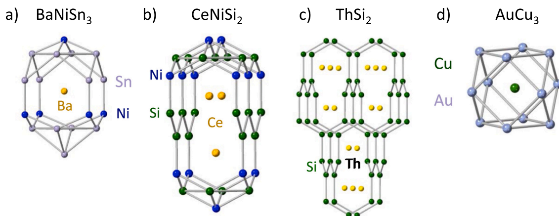
Fig. 1. The crystal structures of the structure types (a) \text{BaNiSn}_3 , (b) \text{CeNiSi}_2 , (c) \text{ThSi}_2 , and (d) \text{AuCu}_3 are shown to illustrate the relationship between the stacking units of the homologous series \text{Ln}_{n+1}\text{M}_n\text{X}_{3n+1} ( \text{Ln} = lanthanide, M = transition metal, and X = tetrel).
