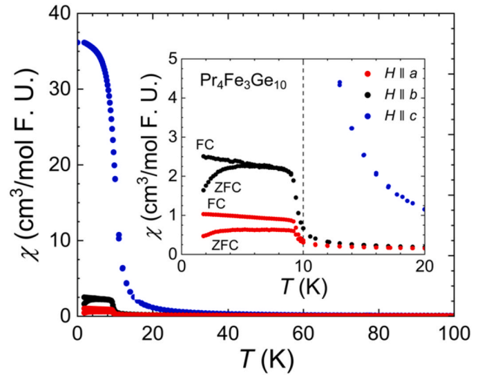
Fig. 5. The magnetic susceptibility (measured at 0.1 T) as a function of temperature is shown for Pr 4 Fe 3 Ge 10 . Along the a (red circles), b (black circles), and c (blue circles) crystallographic direction. The inset contains a zoomed region to highlight the transition temperature at 10 K and the bifurcation along the a - and b -direction.
