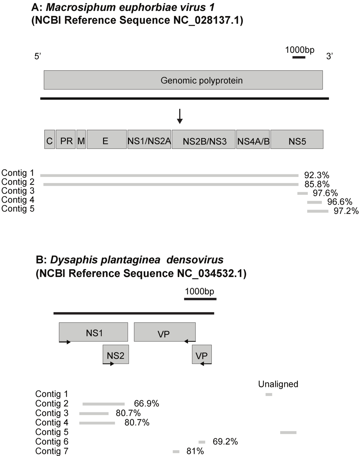
Fig. 2 Assembled M. euphorbiae transcriptome contigs aligning to previously a described insect Flavivirus (A) and an Ambidensovirus (B)
