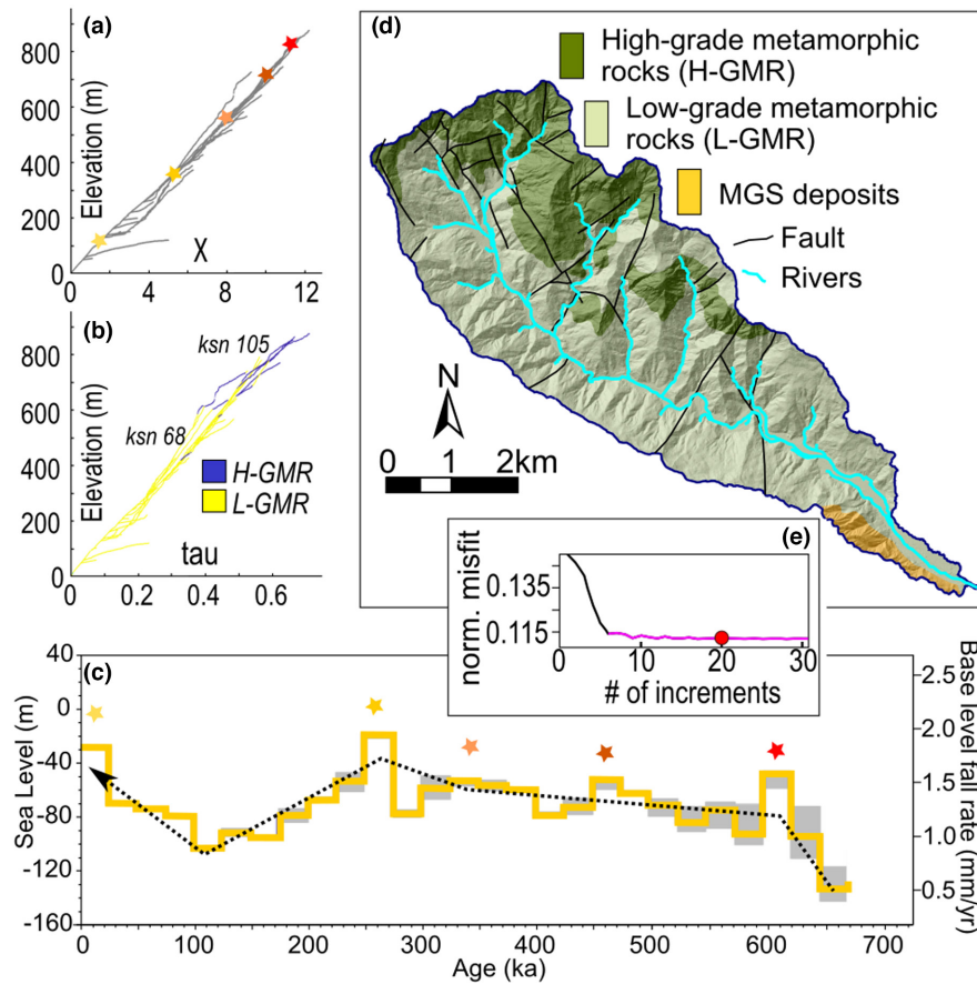
FIGURE 7 (a) \chi -elevation plot (Chi plot) of the Pagliara basin's watershed. The grey lines represent the observed streams profiles. The coloured stars indicate the location of change in k_{sn} , corresponding to the slope change of the modelled long profile in the \chi -elevation space (knickpoint). These knickpoints are paired with the corresponding peaks in the base level fall rate-time plots shown in (c); (b) tau-elevation plot coloured basing on the different rock types, high-grade (H-GMR) and low-grade (L-GMR) metamorphic rocks; (c) step plot showing the Pagliara watershed's long profile inversion results for the reconstruction of the base level fall history encoded in the geomorphic record, obtained using the values in bold in Table 5. The grey shaded portion of the plot shows the misfits of the inversion derived from a total of 1000 iterations run by a Monte Carlo approach; (d) geological map of the Pagliara watershed, also showing the analysed drainage network; (e) results of the sensitivity test run to find a reliable number of \chi increments to discretize the inverted river long profiles. The plot shows a wide zone of low misfit when the long profiles are inverted using >10–15 increments with the minimum misfit provided by discretizing the profile in 20 increments. Each increment corresponds to a \chi -interval of ca. 300.
