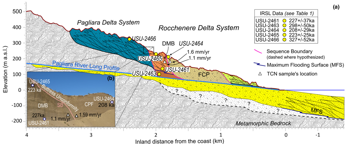
FIGURE 5 (a) Stratigraphic model of the Pagliara fan-delta showing the relationships between the different allostratigraphic units. IRSL ages (circles) and TCN paleo-erosion rates (triangles) are keyed into their sampling sites. The resulting IRSL ages and relative errors are also reported. (b) Photo of the quarry highwall annotated with specific features depicted in (a), showing the buttress unconformity that separates the DMB facies of samples USU-2461 and USU-2465 from the fluvial/coastal plain deposits sampled at site USU-2464 (see (a) for reference).
