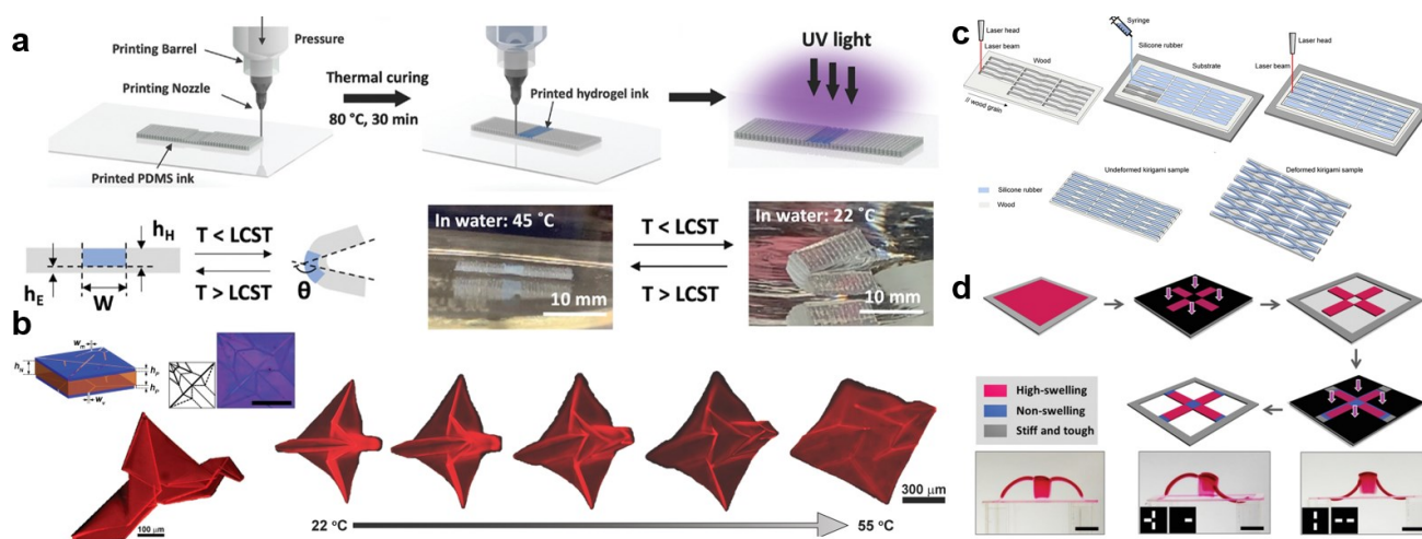
Fig. 11 Strategies for fabricating hinges and cutouts in origami and kirigami, respectively. (a) Schematic depicting Direct Ink Writing (DIW) 4D printing fabrication technique utilized for printing hinges that allow for origami-inspired folding. Reproduced with permission. 224 Copyrights 2022, Wiley-VCH. (b) Photolithography used to pattern hydrogel sheet with UV light which creates the hinges on the hydrogel sheet which exhibits reversible folding and unfolding of a Randlett's bird when exposed to different temperatures. Reproduced with permission. 239 Copyrights 2015, Wiley-VCH. (c) Cured hydrogel sliced into a kirigami-inspired structure using a laser cutter. Reproduced with permission. 255 Copyrights 2019, Springer Nature. (d) Photolithography mask used during the hydrogel curing process to create kirigami-inspired cut outs. Reproduced with permission. 304 Copyrights 2020, Wiley-VCH.
