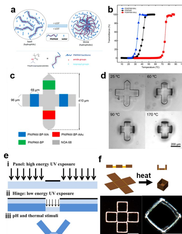
Fig. 12 (a) Schematic illustration of thermos-responsive LCST behavior of PNIPAM. Reproduced with permission. 312 Copyrights 2020, Royal Society of Chemistry. (b) Temperature dependence of transmittance at 515 nm for PNIPAM copolymer solutions in ionic liquid at a heating rate of 1 °C/min (c) Schematic illustration of the design for a sequential self-folding PNIPAM-based hydrogel sheet in the plan view (d) Optical images of a self-folding micropatterned PNIPAM-based hydrogel sheet in ionic liquid at different temperatures throughout heating. Reproduced with permission. 316 Copyright 2017, American Chemical Society. (e) Schematic of P(NIPAM-AAc) hydrogel strip with (i) thick, fully crosslinked panel and (ii) thin, gradient crosslinked hinge. (iii) Schematic deformation of hydrogel strip under Ph and thermal stimuli (f) Schematic and optical images of temperature responsive self-folding. Reproduced with permission. 318 Copyright 2014, IOP Publishing.
