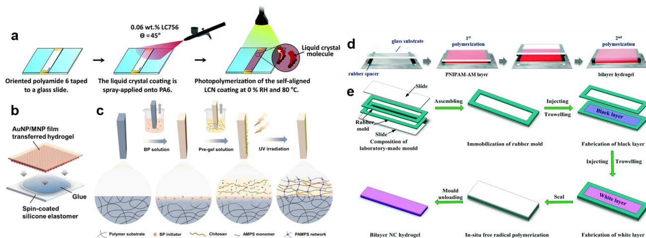
Fig.8 Fabrication of composite bilayer hydrogel structures using different coating techniques: (a) spray coating of liquid crystal elastomer (LCN) onto the surface of polyamide 6 (PA6) using a spray gun. Reproduced with permission. 259 Copyrights 2018, Royal Society of Chemistry. (b) AuNP/MNP film transferred onto spin-coated temperature-responsive hydrogel attached to spin-coated silicon elastomer; Reproduced with permission. 260 Copyrights 2021, American Chemical Society. (c) dip coating fabrication technique used for double-network hydrogels. Reproduced with permission. 265 Copyrights 2022, American Chemical Society Publications. Casting fabrication process for composite bilayer hydrogel systems: (d) casting bilayer hydrogels with rubber spacers where the precursor solution is injected in between two glass slides; Reproduced with permission. 268 Copyrights 2018, Royal Society of Chemistry. (e) casting bilayer hydrogels inside customized laboratory made molds. Reproduced with permission. 270 Copyrights 2018, Royal Society of Chemistry.
