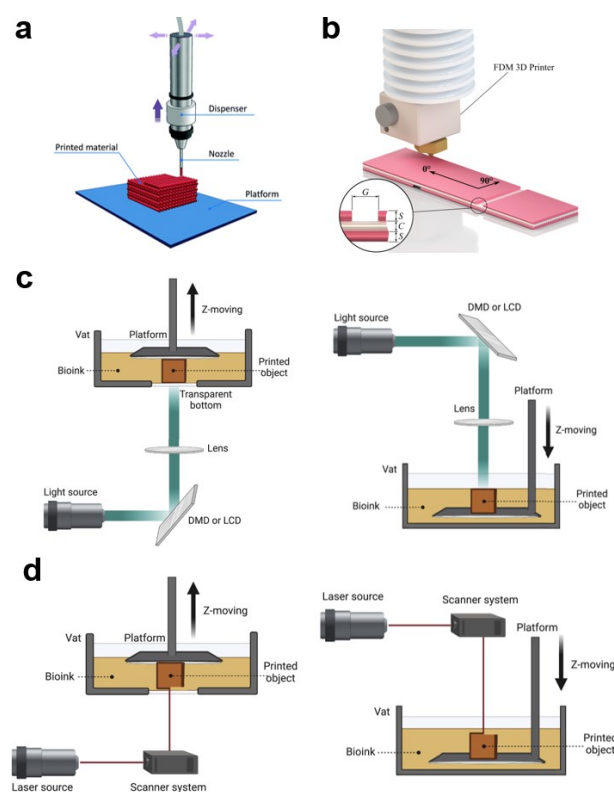
Fig.9 3D printing fabrication strategies. (a) Schematic of Direct Ink Writing (DIW) printing where the hydrogel exits from a syringe and its nozzle using pressure or mechanical extrusion. Reproduced with permission. 288 Copyrights 2016, Royal Society of Chemistry. (b) Schematic of Fused Filament Fabrication (FFF) where thermoset plastics are heated through a nozzle and extruded. Reproduced with permission. 283 Copyrights 2019, Elsevier. (c) Bottom-down approach and top-down approach Digital Light Processing (DLP) printing. Bottom-down DLP has the light source projected by a digital mirror device (DMD) or a liquid crystal display (LCN) from the bottom into the vat of precursor solution, whereas top-down DLP has the light source projected from the top of the vat. (d) Schematics of both the bottom-down and top-down approach of stereolithography (SLA) printing. Bottom-down SLA where a laser directed toward the bottom of the vat and top-down SLA where a laser is directed at the top of the vat. Reproduced with permission. 290 Copyrights 2023, Elsevier.
