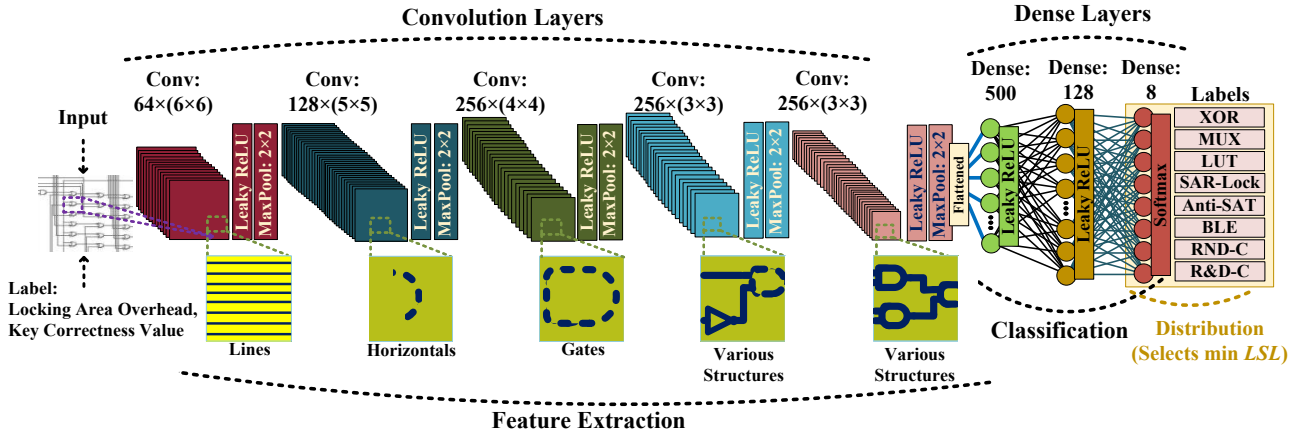
Figure 3: CoLA structure
