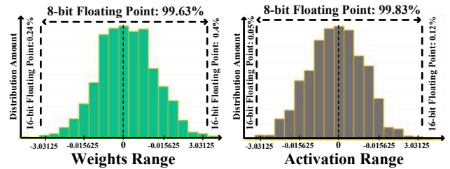
Figure 6: Distribution of the weights and activation values
