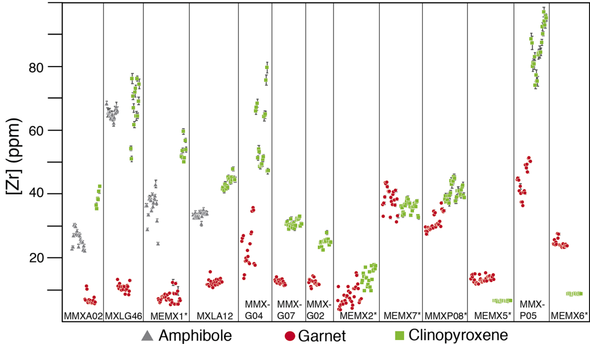
Fig. 8. In situ (LA-ICP-MS) Zr concentrations in rock-forming phases. Samples are in order (left to right) of increasing temperature from thermobarometry (Bloch et al., 2017; Ziemann et al., 2023). Asterisks indicate samples analyzed for Zr isotopes within mineral fractions.
