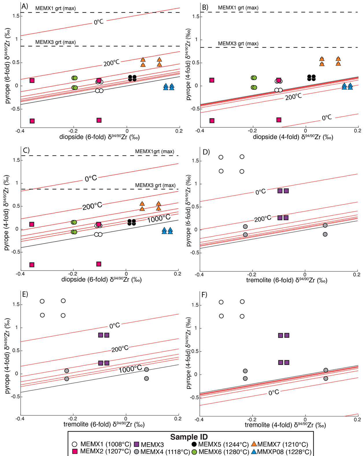
Fig. 11. Measured mineral fraction \delta^{94/90}\text{Zr} values compared to isothermal \delta^{94/90}\text{Zr} equilibrium ( ab initio ) predictions from Chen et al. (2020) for garnet, clinopyroxene, and amphibole end-members. Black line denotes the 1:1 line. Panels show different possible combinations of Zr substitutions in tetrahedral and octahedral crystallographic sites. Four points are plotted for each cumulate sample, showing the four possible combinations of maximum-minimum \delta^{94/90}\text{Zr} values of co-existing mineral fractions [e.g., four pink squares in panel A represent 1) max \delta^{94/90}\text{Zr}_{\text{grt}} vs. max \delta^{94/90}\text{Zr}_{\text{cpx}} , 2) max \delta^{94/90}\text{Zr}_{\text{grt}} vs. min \delta^{94/90}\text{Zr}_{\text{cpx}} , 3) min \delta^{94/90}\text{Zr}_{\text{grt}} vs. max \delta^{94/90}\text{Zr}_{\text{cpx}} , and 4) min \delta^{94/90}\text{Zr}_{\text{grt}} vs. min \delta^{94/90}\text{Zr}_{\text{cpx}} for sample MEMX2]. Dashed lines in panels A-C show the maximum \delta^{94/90}\text{Zr} of garnet for the two samples from which clinopyroxene fractions were not recovered. (For interpretation of the references to colour in this figure legend, the reader is referred to the web version of this article.)
