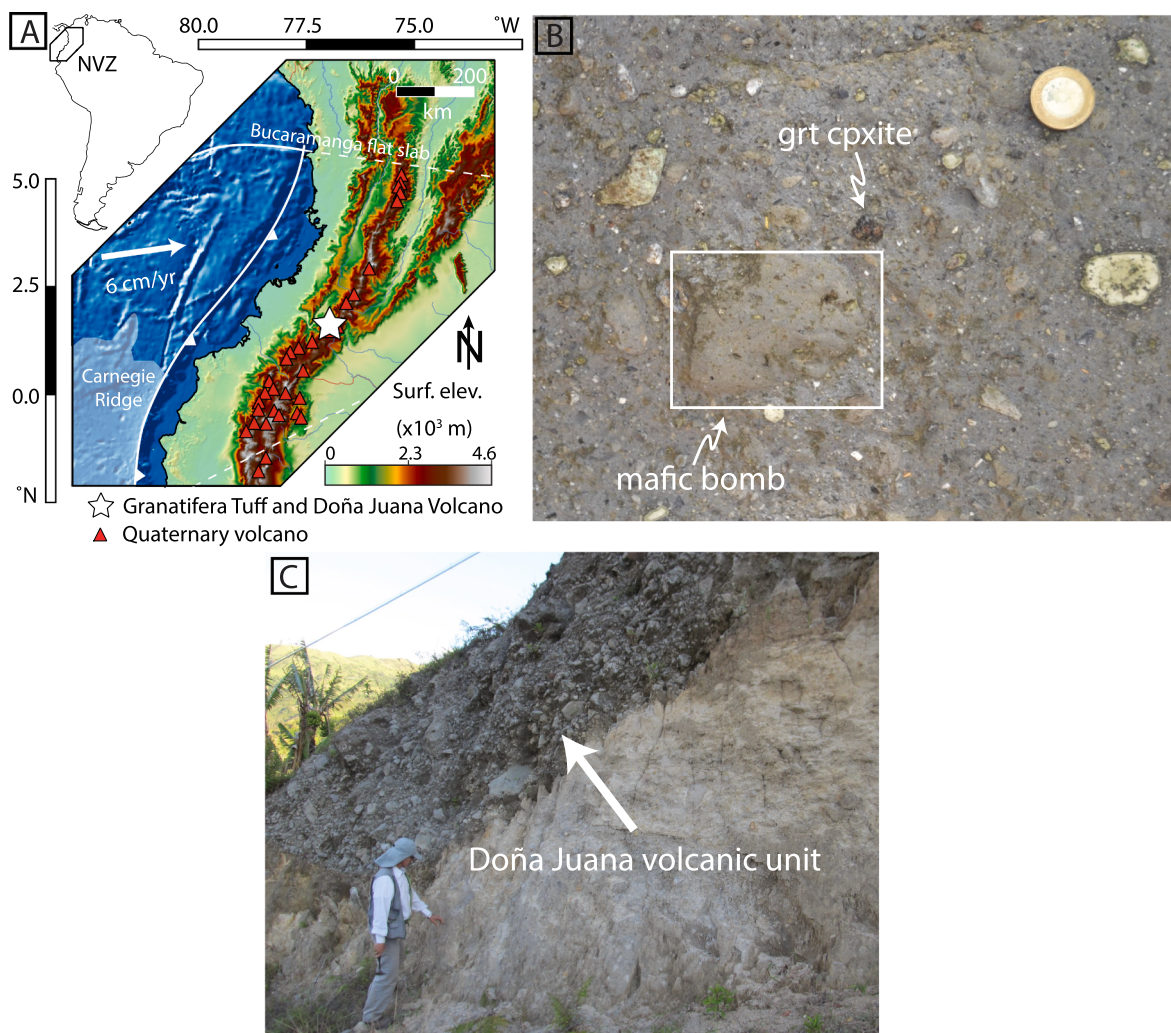
Fig. 1. A) Map of the Andean Northern Volcanic Zone (NVZ) showing the location of the Granatifer Tuff and the Doña Juana Volcanic Complex. B) Field photo of the Granatifer Tuff containing a garnet clinopyroxenite cumulate and a mafic bomb. C) Typical dacitic unit of the Doña Juana Volcanic Complex, the felsic volcanic rocks measured in this study.
