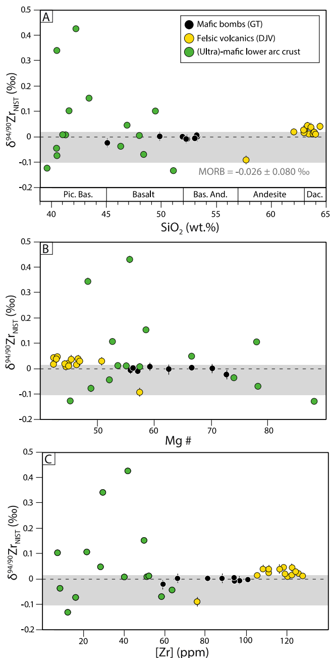
Fig. 3. Whole rock Zr isotopic composition ( \delta^{94/90}\text{Zr} = [({}^{94/90}\text{Zr}_{\text{sample}}/{}^{94/90}\text{Zr}_{\text{NIST}}) - 1] \times 10^3 ) vs. A) \text{SiO}_2 wt. %, B) Mg#, and C) [Zr] for mafic and felsic extrusive volcanic rocks as well as garnet clinopyroxenite ( \pm amphibole) cumulates. Error bars are smaller than symbols where not visible, see Table 1. Range of MORBs (gray field) is from Inglis et al. (2019), recalculated relative to the NIST standard from the IPGP-Zr standard ( \delta^{94/90}\text{Zr}_{\text{NIST}} = -0.055 \pm 0.002 ‰; Klaver et al., 2021).
