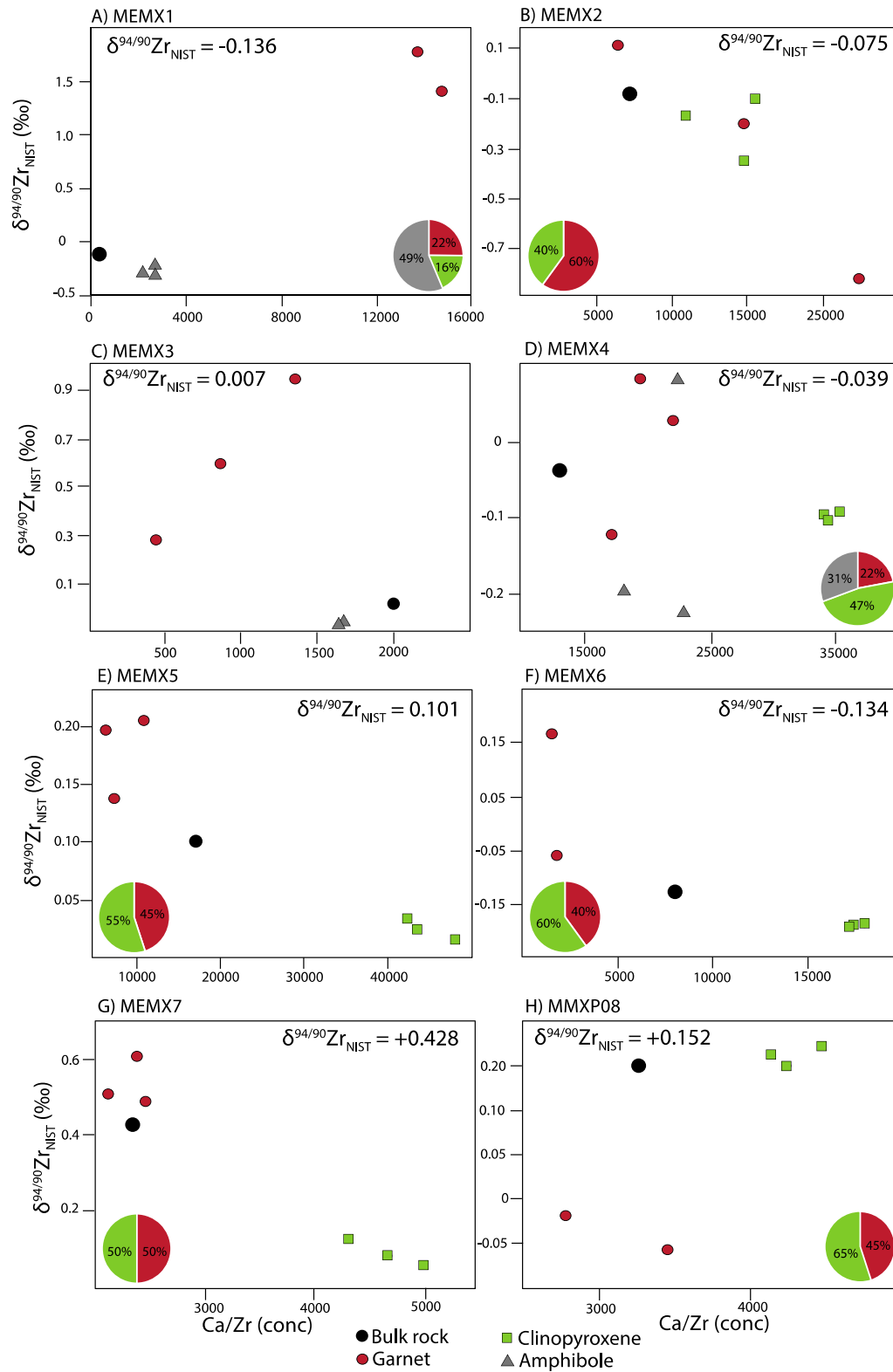
Fig. 6. Zirconium isotopic compositions of bulk rock and mineral fractions from eight garnet clinopyroxenite (±amphibole) cumulates vs. Ca/Zr ratios. Ca was chosen for the numerator because this is a major element that varies significantly between garnet, clinopyroxene, and amphibole, and Zr was chosen in the numerator to evaluate if the \delta^{94/90}\text{Zr} variations in each sample can be explained by simple two- or three-component mixing. Pie chart insets represent the modal abundances of major phases. Insets of \delta^{94/90}\text{Zr} values indicate the bulk rock isotopic compositions.
