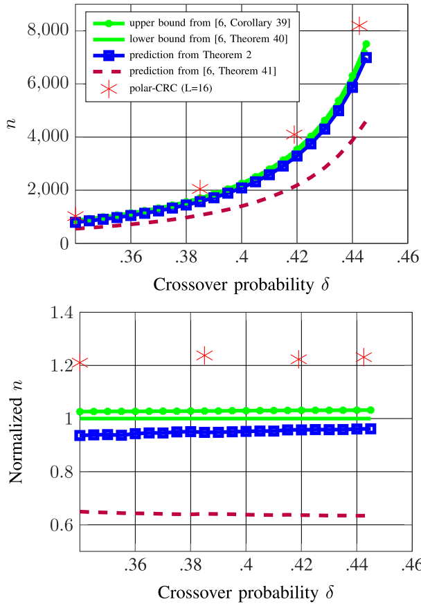
Fig. 2. Comparison for low-capacity BSC. The number of information bits is k = 40 and the target error probability is p_e = 0.01 . For the lower plot, with the same legend entries as the upper plot, all the blocklengths n in the upper plot are normalized by lower bound given by [6, Th. 40].
