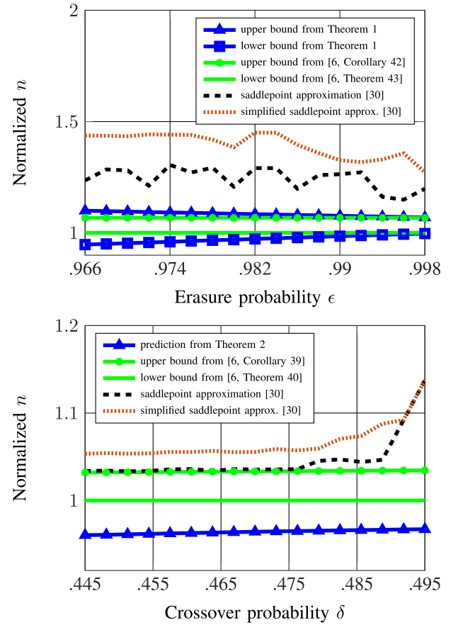
Fig. 3. Sending k = 40 information bits over BEC (up) and BSC (down) in the low-capacity regime for the target error probability p_e = 0.01 to compare our approximations from Theorem 1 and Theorem 2 or equivalently Corollary 1 with saddlepoint approximations [30].
