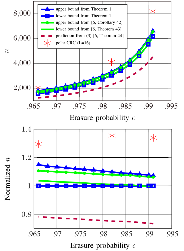
Fig. 1. Comparison for low-capacity BECs. The number of information bits is k = 40 and the target error probability is p_e = 0.01 . For the lower plot, with the same legend entries as the upper plot, all the blocklengths n in the upper plot are normalized by the value of the lower bound obtained from Theorem 1.
