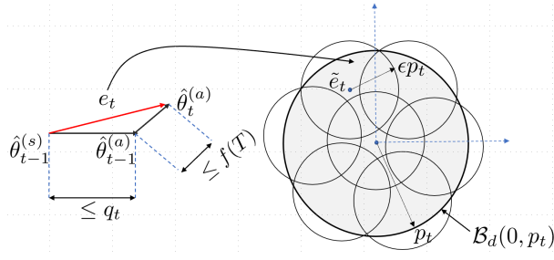
Figure 2: Illustration of the encoding technique in Algorithm 1. The agent computes the innovation signal e_t that belongs to \mathcal{B}_d(0, p_t) with high probability. An \epsilon p_t -net of \mathcal{B}_d(0, p_t) is constructed, and the center \tilde{e}_t of the ball containing e_t is decoded by the server.
