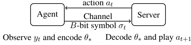
Figure 1: At each round t , the action a_t played by the server is sent to the agent without any loss of information. The agent then observes a reward y_t as per Eq. (1), encodes an estimate of the model \theta_* , and transmits the encoded symbol \sigma_t back to the server under the B -bits per round channel constraint. The server performs decoding and plays the next action a_{t+1} .
