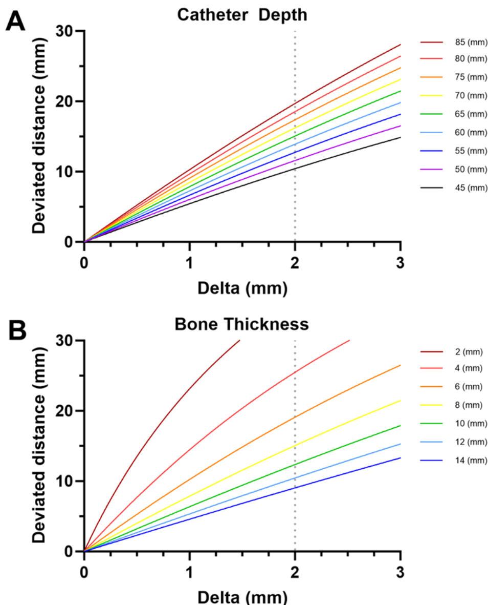
FIG. 4. Effect of catheter depth and bone thickness on deviated distance as a function of the difference between the craniotomy diameter and the catheter diameter (delta). Plots derived from the equation in Fig. 3 were generated as a function of the delta term. A catheter diameter of 3.4 mm was assumed for both plots, while a bone thickness of 8 mm was assumed for the various depths (A) and a catheter depth of 75 mm was assumed for various bone thicknesses (B). A vertical dashed line at 2.0 mm is plotted, representing the delta of a standard Codman twist-drill bit (5.4 mm) and Bactiseal EVD catheter (3.4 mm).
