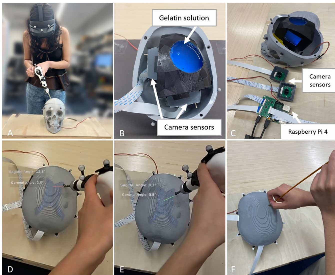
FIG. 1. Sensing-integrated skull phantom for mixed reality-guided craniostomy. A: A sensing-integrated skull phantom for optical marker-based tracking of the twist-drill and mixed reality overlay of ventricular anatomy was created. B and C: The intracranial phantom mold was filled with 8% gelatin ( B ), and ventriculostomy catheter placement was tracked via camera sensors integrated into Raspberry Pi 4 microcontrollers ( C ). D: Drill trajectories were overlaid onto the phantom in red with degrees of deviation from the optimal trajectory in the coronal and sagittal planes displayed. E: When the trajectory was < 1^\circ from optimal, the holographic trajectory changed to green. F: Following the mixed reality-guided craniostomy, the ventriculostomy catheter was advanced.
