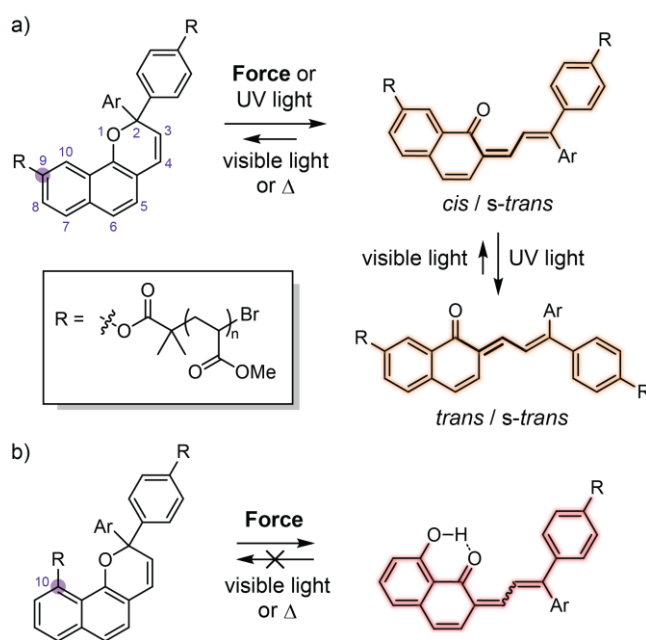
Scheme 1. Reactions of 2H-naphthopyran-containing poly(methyl acrylate) polymers and the structures of the merocyanine dyes produced upon mechanochemical or photochemical activation.
