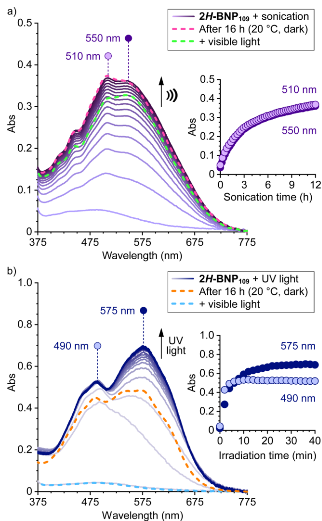
Figure 2. (a) Ultrasound-induced mechanochemical activation (12 h, 20 °C) of 2H-BNP 109 generates a product mixture with absorption maxima at approximately 510 and 550 nm. After incubation at 20 °C for 16 h in the dark, the spectrum remains essentially unchanged. Irradiation with 565 nm light (150 min) results in minimal bleaching. (b) Photoirradiation of 2H-BNP 109 with 365 nm UV light (40 min, 20 °C) generates a product mixture with absorption maxima at ~490 and 575 nm. Some attenuation of the absorbance is observed after 16 h in the dark (20 °C). Irradiation with 565 nm light (180 min) results in nearly complete bleaching. Insets show time-dependent absorbance at the specified wavelengths.
