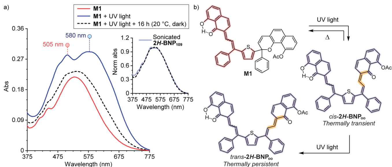
Figure 4. (a) Photoirradiation of M1 with UV light (345 nm, 8 min) results in a bathochromic shift in absorption with maxima at 505 and 580 nm. Upon cessation of photoirradiation and 16 h in the dark (20 °C), the spectrum evolves to closely match the final absorption spectrum obtained upon sonication of 2H-BNP 109 (inset). (b) Reaction scheme illustrating the formation of a mixture of thermally transient and persistent bis-merocyanine isomers with cis and trans exocyclic alkene geometry on the ester-containing subunit upon exposure of M1 to UV light.
