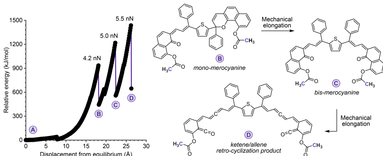
Figure 5. Density functional theory (DFT) calculations using the constrained geometries simulate external force (CoGEF) method performed on a truncated model of 2H-BNP predict an unusual retro-cyclization reaction upon extended mechanical elongation to generate two sets of ketene and allene motifs. Structures are shown that correspond to the computed products of pyran ring opening (B and C) and the unusual retro-cyclization reaction (D) on the CoGEF profile. Calculations were performed at the B3LYP/6-31G* level of theory. The purple carbon atoms of the terminal methyl groups define the distance constraint.
