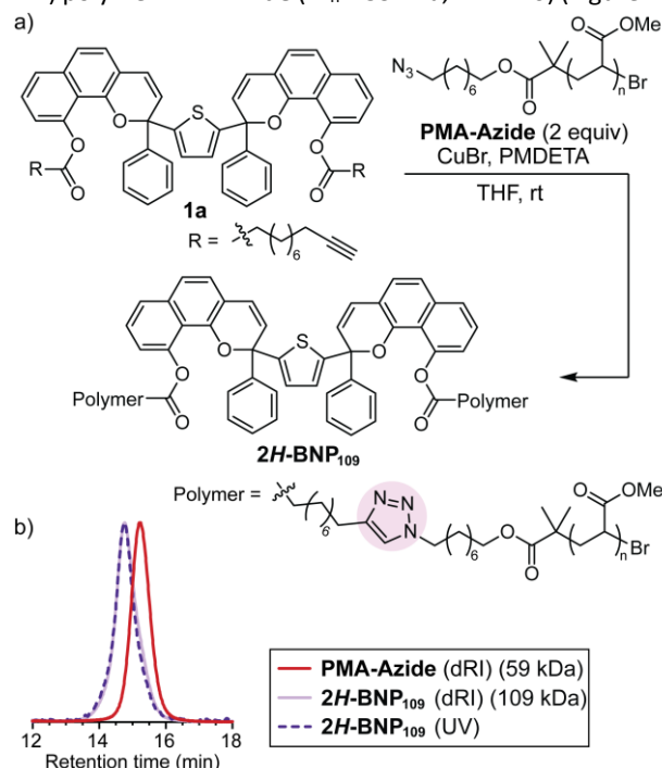
Figure 1. (a) Synthesis of a poly(methyl acrylate) polymer (109 kDa, \bar{D} = 1.17 ) containing a chain-centered 2H -bis-naphthopyran mechanophore unit via CuAAC. (b) Characterization by GPC-MALS with differential refractive index (dRI) and in-line UV detection (345 nm) confirms 2H -bis-naphthopyran functionalization near the chain center.
