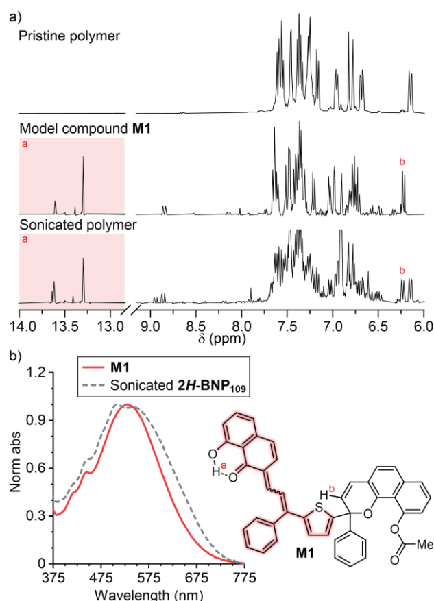
Figure 3. (a) Characteristic resonances in the 1 H NMR (THF- d 8 , 400 MHz) spectrum of model compound M1 are also observed in the product mixture generated from ultrasound-mediated mechanical activation of 2H-BNP 109 . (b) The absorption spectrum generated during the sonication of 2H-BNP 109 is not consistent with pristine M1 . The long wavelength feature is bathochromically shifted from the absorption maximum of M1 .
