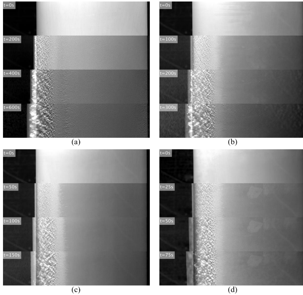
Figure 3: Dynamic Ice Accretion Process on the surface of the wind turbine blade model for Rime Ice at V_{\infty} = 40 m/s, T = -15 °C at (a) LWC = 0.5 g/m 3 (b) LWC = 1 g/m 3 (c) LWC = 2 g/m 3 (d) LWC = 4 g/m 3
