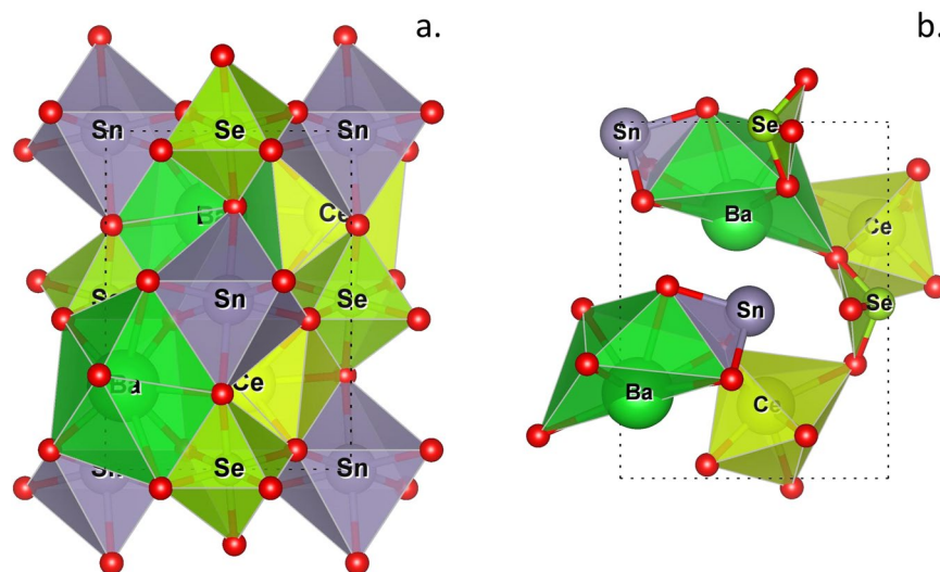
Fig. 4 (a) The perovskite structure generated by SPuDS in the a^-b^+a^- Glazer tilt for the theoretical perovskite \text{BaCeSnSeO}_6 . (b) The non-perovskite, DFT-optimized structure of \text{BaCeSnSeO}_6 , which no longer has an interconnected network of \text{SeO}_6 and \text{SnO}_6 octahedra following DFT optimization.
