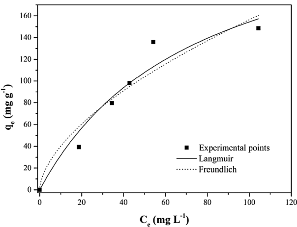
Figure 11. The adsorption isotherms curve of MO by 1.5% PEG-GO/CS.
