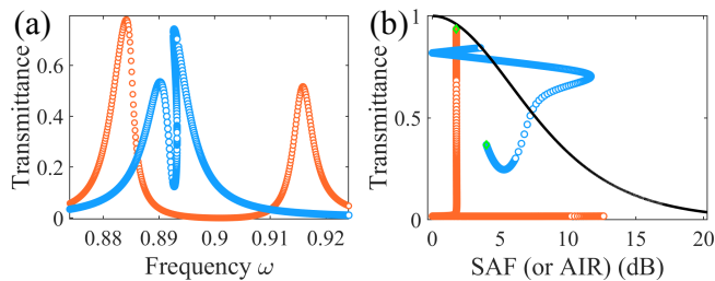
FIG. 3. (a) Two examples of overlapping (blue circles) and isolated (orange circles) resonance scenarios using NLRMT modeling. (b) The (maximum) transmittance vs. SAF for the two cases shown in (a) for a fixed value of the frequency ( \omega = 0.884 for the isolated resonance case and \omega = 0.892 for the overlapping resonance case) of the incident wave. The loss increases from zero (green diamonds). The system that supports overlapping resonances breaks the lossless bound Eq. (8) (solid black line) at certain loss values. For details see SM Sec. J.
