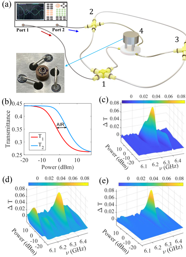
FIG. 1. (a) A microwave tetrahedron graph. The coaxial cables are connected by T or double T-junctions at each of the vertices n = 1, 2 , and 3. Vertex N = 4 consists of three kink antennas coupling to a cylindrical dielectric resonator that is inductively coupled to a ring antenna which is short-circuited with a nonlinear diode (see left inset). (b) Measured transmittance T_1 (from port 1 to port 2) and T_2 (from port 2 to port 1) at a fixed frequency ( \nu = 6.327 GHz) as a function of the input power showing asymmetric transport. (c)-(e) The transmittance difference \Delta T \equiv T_2 - T_1 for an incident wave (of the same amplitude and frequency) as a function of frequency and input power. (c) Experimental data; Simulations using (d) a simple graph; and (e) a resonant-graph modeling.
