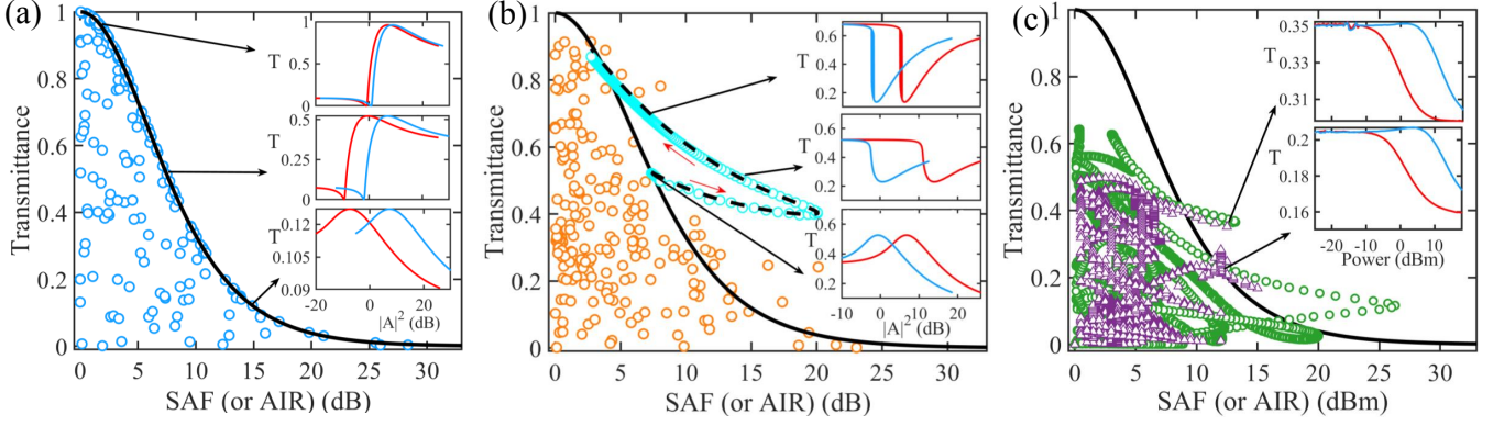
FIG. 2. Transmittance versus structural asymmetry factor (SAF) or asymmetric intensity range (AIR). (a) Lossless graph. The insets show the transmittances versus input intensity from each of the two leads (red and blue lines) for three different SAF graph configurations. (b) Lossy graph with losses on node n_0 = 3 . The light blue circles indicate maximum transmittance for a graph configuration with increasing loss (along the direction of the red arrow) on node 3. The insets correspond to different losses for a fixed graph configuration. (c) Measurements (purple triangles) and simulations (green circles) for an ensemble of graphs with bond-losses and a lossy saturable nonlinearity. The ensemble has been generated by interchanging the bonds of the graph. The insets show measurements corresponding to the same SAF but different maximum transmission values. The black solid and dashed lines in (a-c) are theoretical predictions while the colored circles are simulations occurring at various wavelengths and graph configurations. The data acquisition has been performed for three different graph configurations and for a frequency range \nu \in [6.1 \text{ GHz}, 6.5 \text{ GHz}] with a resolution of \delta\nu = 0.4 \text{ MHz} .
