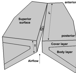
Figure 1: The three-dimensional vocal fold model and key geometric control parameters, including the vocal fold length L along the anterior-posterior direction, vertical thickness of the medial surface T , and the initial glottal angle \alpha .
