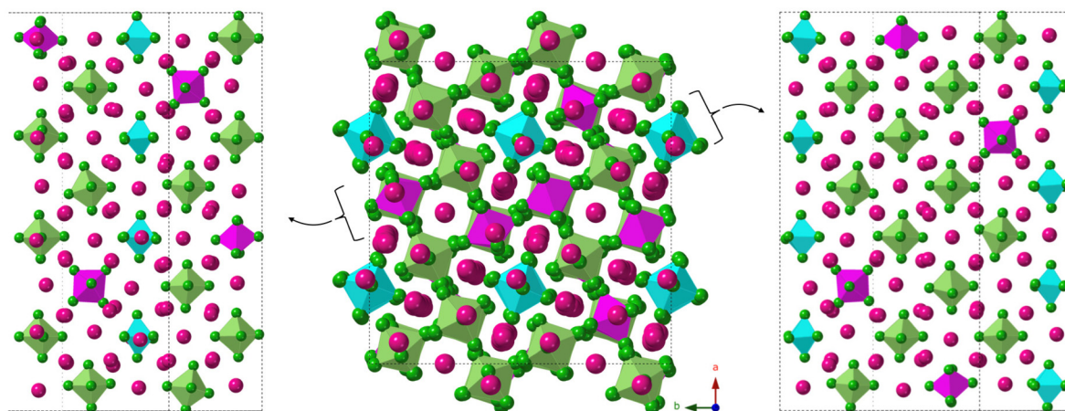
Fig. 5 Structure of t - \text{Rb}_3\text{GaF}_6 showing the view down the c -axis and two individual planes of polyhedra. Rb atoms are shown in pink, the three different orientations of Ga polyhedra in blue, pink and green, and F atoms in green.
