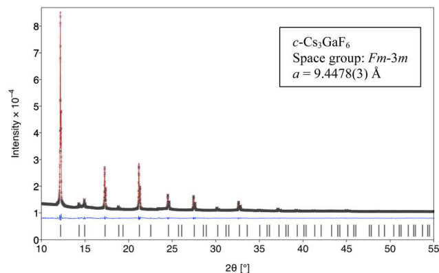
Fig. 8 Rietveld refinement plot of \text{Cs}_3\text{GaF}_6 at 400 °C; red line is Rietveld fit, black X's are observed PXRD (Mo K_\alpha ), blue line is residual, and vertical black ticks are allowed Bragg reflections.
