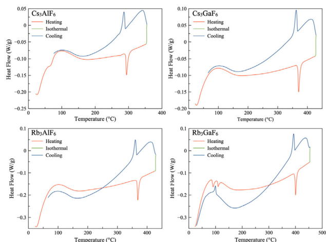
Fig. 6 DSC data for the four compounds showing the heat flow as a function of temperature. Endothermic peaks point down and exothermic peaks point up. No appreciable difference was observed between the monoclinic and orthorhombic \text{Cs}_3\text{MF}_6 compounds so only one is shown.
