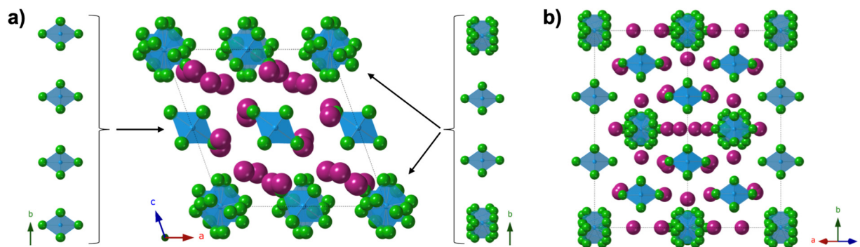
Fig. 2 Structure of m -Cs 3 AlF 6 showing (a) the view down the b -axis and (b) the view down the [1 0 1] direction. Cs atoms are shown in pink, Al polyhedra in blue, and F atoms in green.
