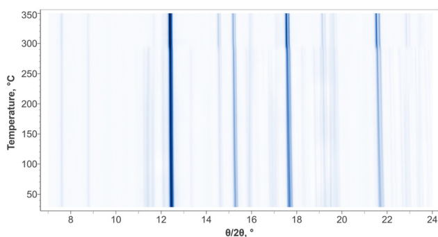
Fig. 7 Waterfall plot of the change in PXRD pattern (Mo K_\alpha ) upon heating for \text{Cs}_3\text{AlF}_6 , highlighting the structure transition from m\text{-Cs}_3\text{AlF}_6 to c\text{-Cs}_3\text{AlF}_6 at 291.2 °C.
