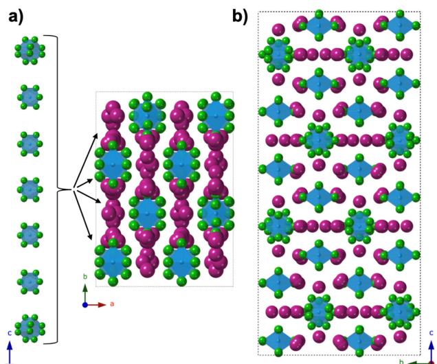
Fig. 3 Structure of o -Cs 3 AlF 6 showing (a) the view down the c -axis and (b) the view down the a -axis. Cs atoms are shown in pink, Al polyhedra in blue, and F atoms in green.
