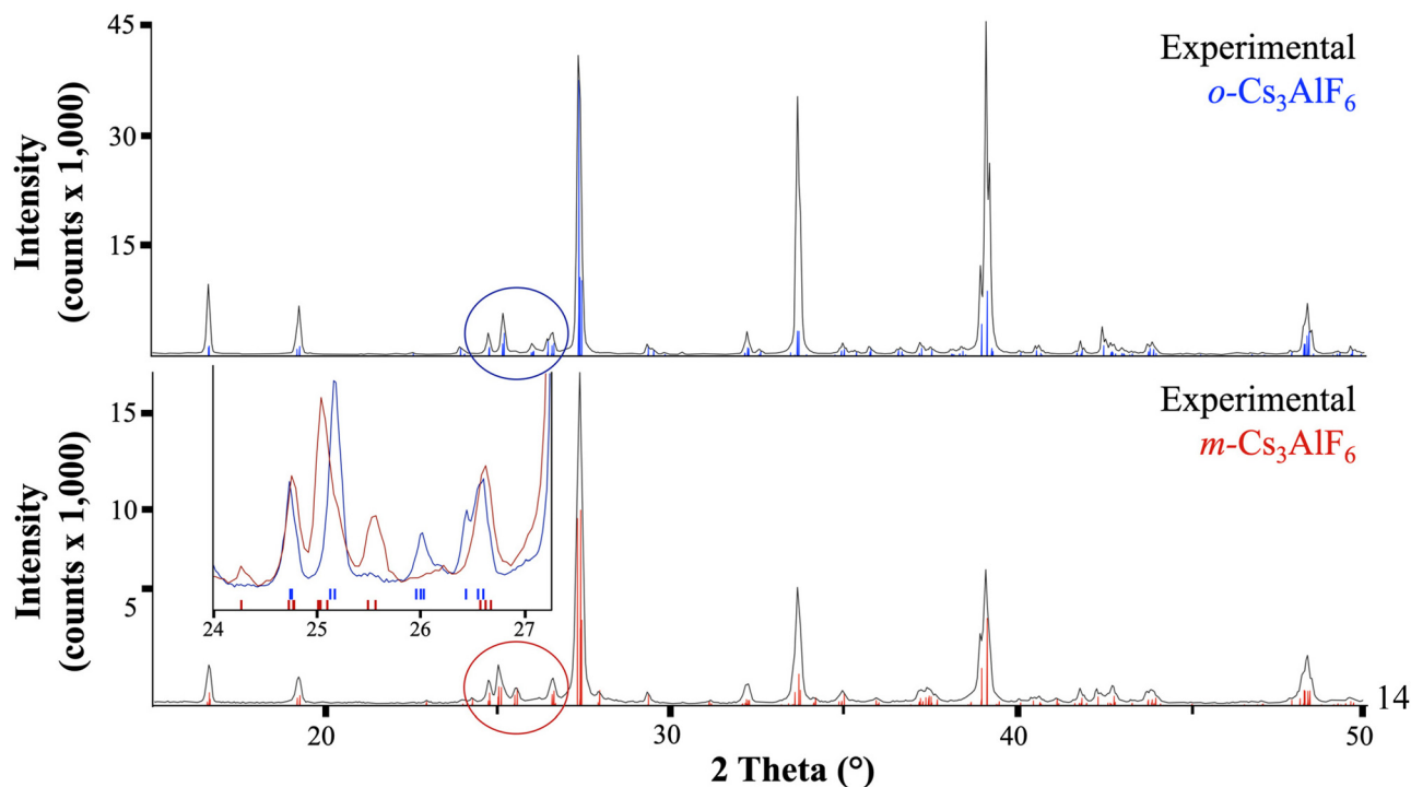
Fig. 4 Powder XRD data (Cu K_{\alpha} ) for m - \text{Cs}_3\text{AlF}_6 and o - \text{Cs}_3\text{AlF}_6 showing the experimental data (black) and patterns calculated from the CIFs (colored). The circled regions are zoomed in the inset to highlight one of the differences between the PXRD patterns of the two polymorphs, where m - \text{Cs}_3\text{AlF}_6 consists of a triplet and a singlet of multiplets, whereas o - \text{Cs}_3\text{AlF}_6 consists of two doublets of multiplets. The small peak at 26.2^\circ is the result of \text{W } L_{\alpha} X-rays that arise when the anode of the X-ray tube is contaminated by the W filament. The difference between the calculated and observed intensities for o - \text{Cs}_3\text{AlF}_6 arise from the use of a low-background slide for this data. See Fig. S18† for data collected in a well sample holder.
