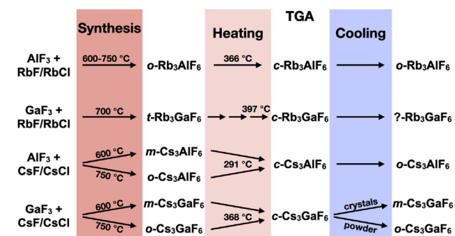
Fig. 1 Schematic summary of the synthesis, structures, and thermal behavior of the reported compounds.
