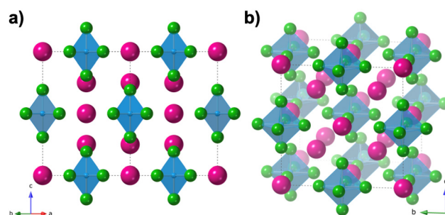
Fig. 9 Structure of c\text{-Cs}_3\text{AlF}_6 showing (a) the view down the [1\ 1\ 0] direction and (b) a view highlighting the double perovskite nature of the structure. Cs atoms are shown in pink, Al polyhedra in blue, and F atoms in green.
