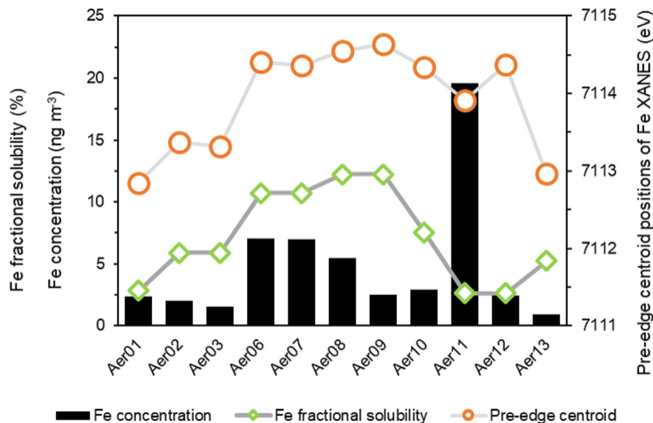
Fig. 4. The variations of pre-edge centroid positions of Fe K-edge XANES, Fe concentrations, and Fe fractional solubility in aerosols during the GN01 cruise (Gao et al., 2019; Marsay et al., 2018). Each pair of the bulk samples (Aer02/03, Aer06/Aer07, Aer08/Aer09, and Aer11/Aer12) corresponded to one size-segregated sample for Fe solubility, as two bulk samples were collected while only one size-segregated sample was collected in the same period of time.
