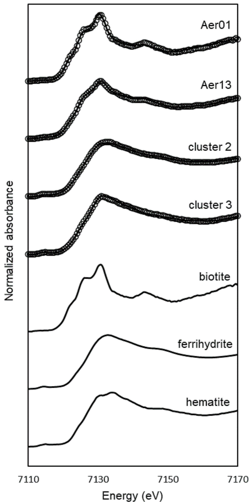
Fig. 3. The results of linear combination fitting in this study. Solid lines and cycles represent the measured spectra and fitting results, respectively.
