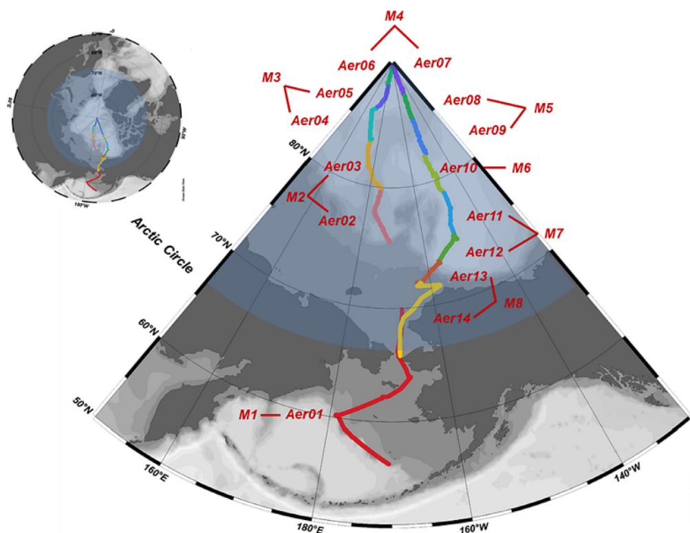
Fig. 1. Cruise track showing the locations of aerosol sampling along the cruise of the US GEOTRACES GN01. AerX and MX represent bulk samples and size-segregated samples, respectively.
