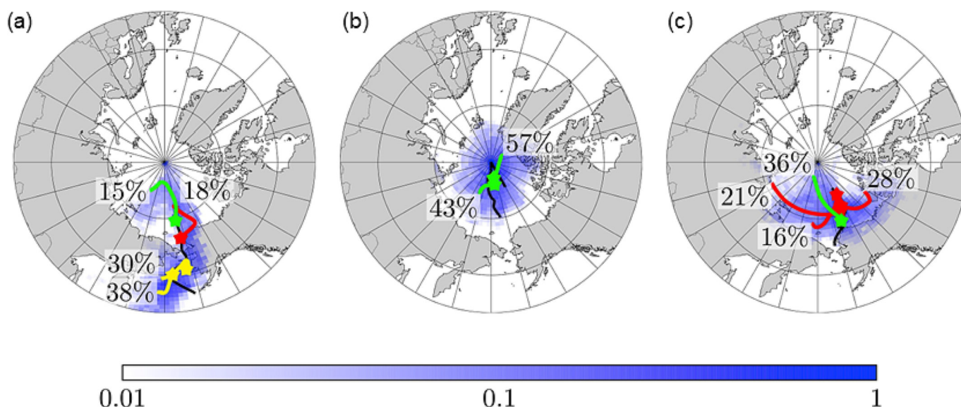
Fig. 2. Results of air mass back trajectory analysis with the NOAA HYSPLIT4 model from Mukherjee et al. (2021) for (a) group 1 samples, (b) group 2 samples, and (c) group 3 samples. The lines with different colors represent the relative impact of distinct sources: type 1: yellow, type 2: green, and type 3: red. The cruise track is shown in black line. The relative spatial frequency of 100 h back-trajectories was calculated and represented by the shades of blue.
