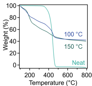
Fig. 4 TGA thermogram of neat SBS, SBS sulfonated at 100 °C for 60 min, and SBS sulfonated at 150 °C for 20 min.
