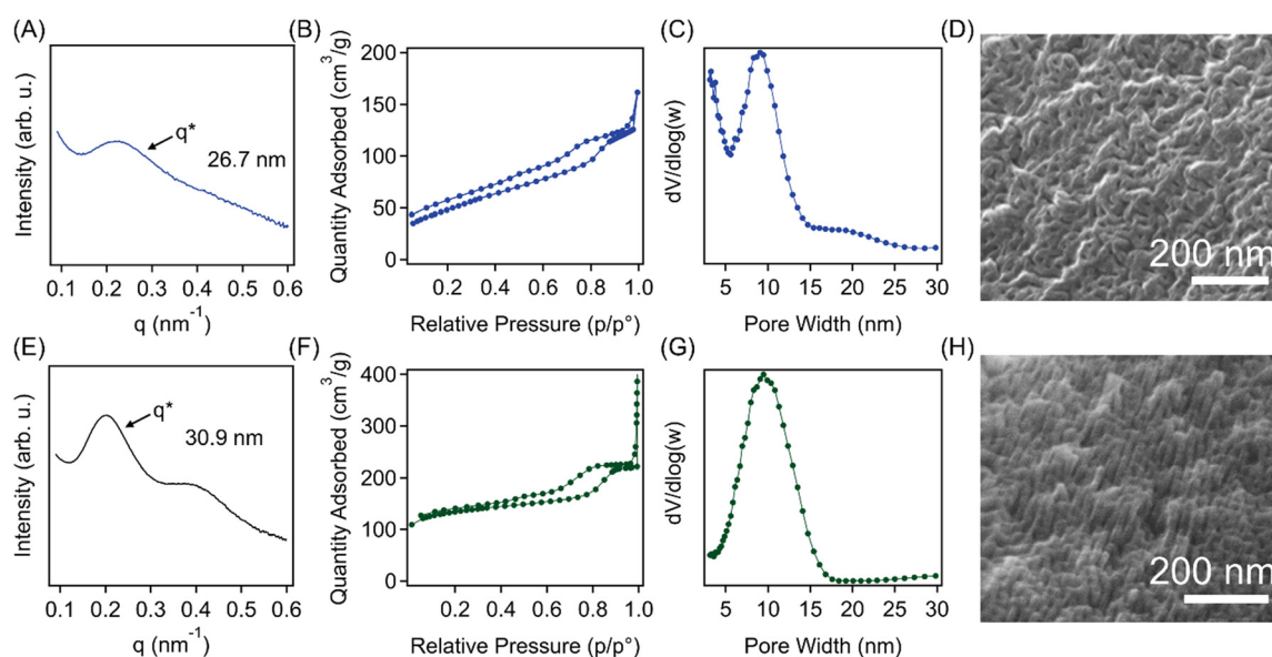
Fig. 6 (A) SAXS pattern, (B) nitrogen physisorption isotherm, (C) NLDFT calculated pore size distribution, and (D) SEM image of the SBS100. (E) SAXS pattern, (F) nitrogen physisorption isotherm, (G) NLDFT calculated pore size distribution and (H) SEM image of the SBS150.
