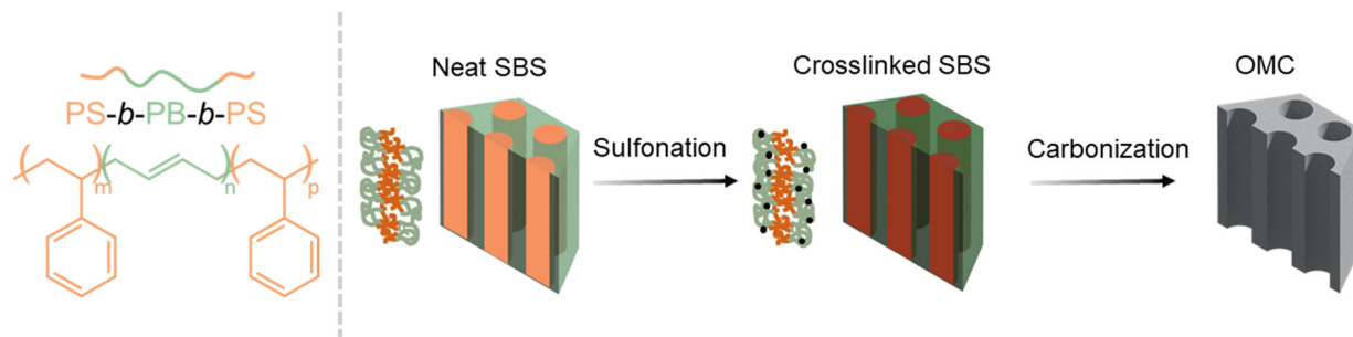
Fig. 1 Representative chemical structure of SBS and a schematic illustration of the sulfonation process used to convert the cylinder forming BCPs to OMCs. As a note, the chemical structure of poly(1,4-butadiene) (PB) segment is simplified, as other isomers may exist.
