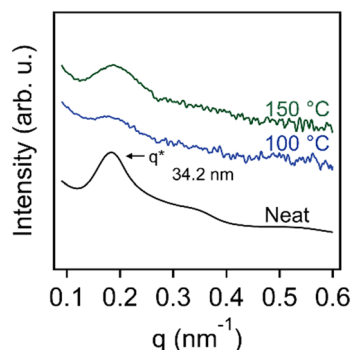
Fig. 3 SAXS results for neat SBS in comparison to samples sulfonated at 100 °C for 60 min and 150 °C for 20 min, respectively.
