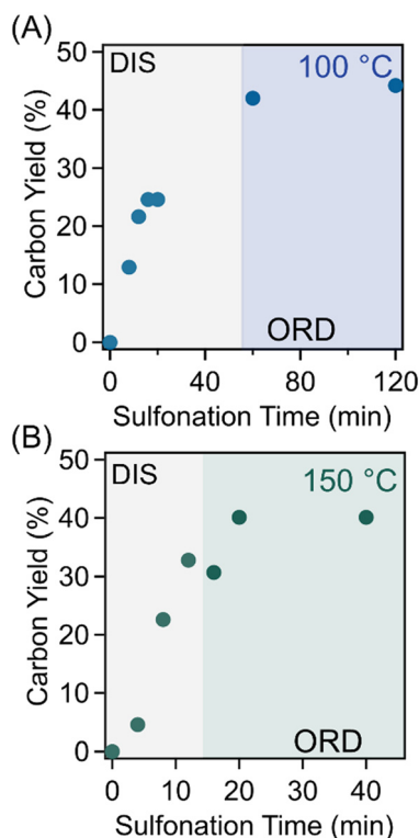
Fig. 5 Carbon yield as a function of sulfonation time for samples sulfonated at (A) 100 °C and (B) 150 °C. Gray shading represents datapoints which do not exhibit ordered pores, while the colored shading represents datapoints which were successfully converted to OMCs.
