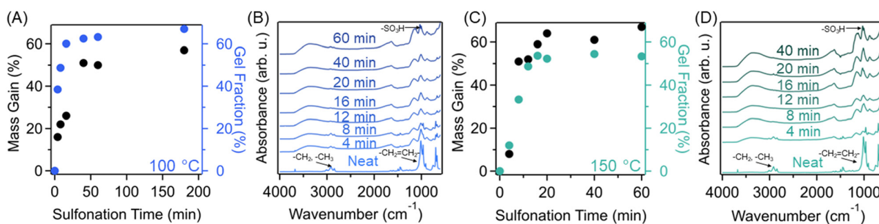
Fig. 2 (A) Mass gain and gel fraction and (B) FTIR spectra of SBS reacted at 100 °C as a function of reaction time. (C) Mass gain and gel fraction and (D) FTIR spectra of SBS reacted at 150 °C as a function of reaction time.
