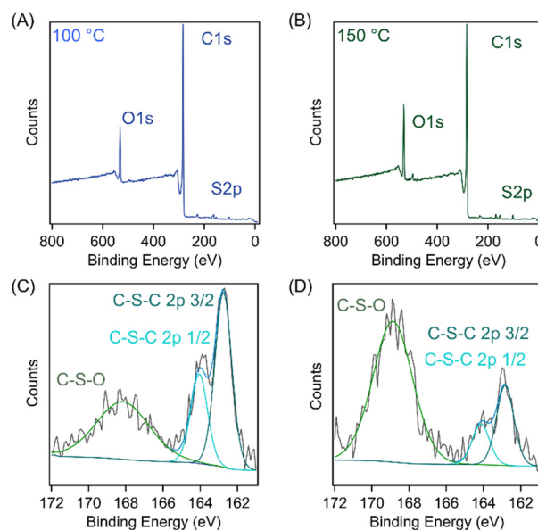
Fig. 7 (A and B) XPS survey scans for SBS100 and SBS 150, respectively. (C and D) Corresponding high resolution S2p scans of SBS100 and SBS150, respectively.
