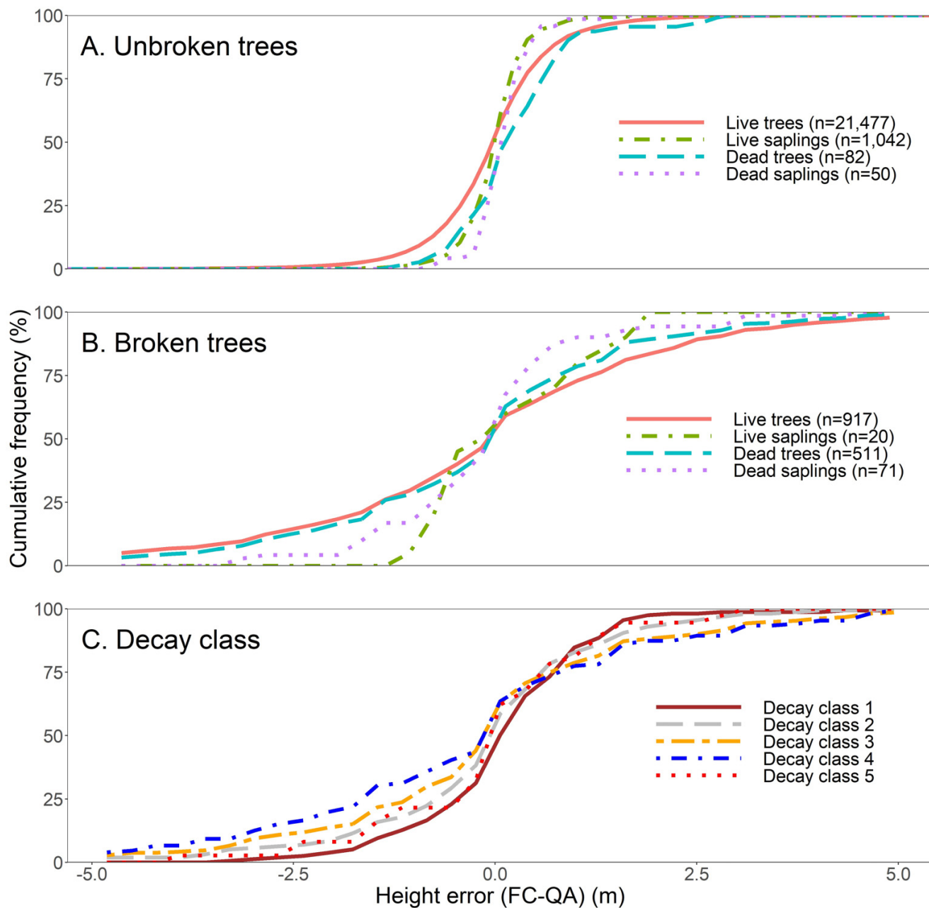
Fig. 3. Tree height measurement errors. (A) Trees not viewed as broken by either the field crew or the quality assurance (QA) crew. (B) Trees viewed as broken by either the field crew or the QA crew. (C) All trees, broken and unbroken, divided by decay class as defined by the QA crew.
