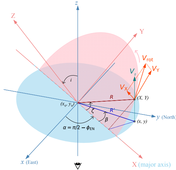
Fig. C.1. Simple schematic diagram for the tilted ring model. The pink semiellipse represents the galaxy plane with a coordinate system of XYZ . The red-based color lines are on or perpendicular to the galaxy plane. The light-blue ellipse presents the sky plane with a coordinate system of xyz . The blue color lines are on or perpendicular to the sky plane. We take the x direction as the east and the y direction as the north. The major axis on the sky plane coincides with the X axis on the galaxy plane. The line-of-sight direction is along the z direction from the bottom to the top. The galaxy plane is inclined with an angle of i (the inclination angle, i.e., the angle between the line of sight and the perpendicular line to the galaxy plane XY ). The data point ( X, Y ) with a distance of R to the center rotates counterclockwise with a rotation velocity of V_{\text{rot}} on the galaxy plane. What we can see is the line-of-sight component V_z of the rotation velocity V_{\text{rot}} . The angle between the major axis on the sky plane and the line connecting the galaxy center ( x_0, y_0 ) and the data point ( X, Y ) is the azimuth angle \zeta . The position angle \phi is defined as the angle counting from the north ( y axis) to the major axis of the receding half on the galaxy plane. After tilting, the data point ( X, Y ), the distance R and the azimuth angle \zeta on the galaxy plane project to (x, y) , R' and \beta on the sky plane.
