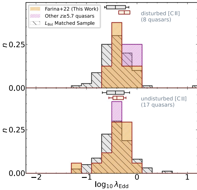
Figure 10. Logarithmic Eddington ratio distributions of the quasars observed at <0''.25 resolution with ALMA by Neeleman et al. (2021). Host galaxies that show disturbed and undisturbed [C II] 158\ \mu\text{m} morphologies are shown in the upper and lower panels, respectively. For the sake of comparison, the Eddington ratios of the luminosity-matched samples are also shown in black. However, note that no information on the hosts is taken into account for the selection of the z \sim 0.3 - 2.3 quasars. The box plots at the top of each panel mark the median values of the various distributions. High-redshift quasars residing in galaxies with a disturbed morphology have a median Eddington ratio higher than those in undisturbed hosts. However, the two distributions do not differ enough to suggest differences between their parent populations. The color code is the same as in Figure 6.
