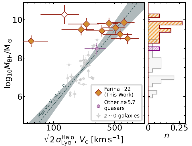
Figure 13. Distribution of z \gtrsim 5.7 quasars in the circular velocity vs. black hole mass plane. Circular velocities are derived from the 1D velocity dispersion of the \text{Ly}\alpha halos considering V_c = \sqrt{2} \sigma_{\text{Ly}\alpha}^{\text{Halo}} . Black hole masses and circular velocities for local galaxies are taken from the review of Kormendy & Ho (2013; gray points). The gray dashed line is the best fit to the z \sim 0 data following the procedure in Volonteri et al. (2011). Histograms in the right panel show the distribution of black hole masses of the high-redshift and local samples. The color code is the same as in Figure 11.
