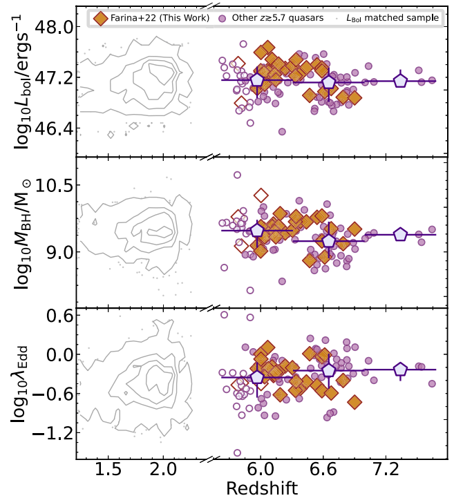
Figure 8. Redshift distribution of (from top to bottom) bolometric luminosities, black hole masses, and Eddington ratios for bright ( M_{1450} < -25.2 mag) z \gtrsim 5.7 quasars (color coded as in Figure 5). Blue pentagons mark median values in three redshift bins. Error bars on the y-axis represent the 16th and the 84th percentiles of the distribution, while on the x-axis they indicate the size of the redshift bin. For comparison, the distribution of the luminosity-matched sample is also shown by gray contours.
