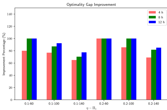
Fig. 8. Optimality Gap Improvement (IEEE 33-Bus system)
