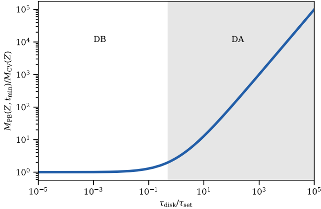
Figure 11. Minimum parent body mass solution relative to the observed mass of pollution in the atmosphere, as a function of the ratio of the disk timescale to the settling time. DAs would be found toward the right, so that the steady-state parent body mass is several times the observed mass in the atmosphere. DBs would be toward the left, where the parent body solution approaches the mass of the polluting metals.
