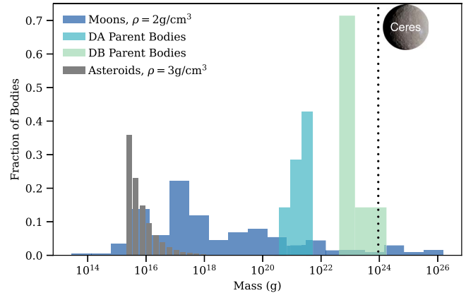
Figure 6. Fraction of bodies in each population with a given mass. Densities of 3 and 2 \text{g cm}^{-3} are assumed to calculate masses for asteroids and moons, respectively. The asteroid curve is derived from Dohnanyi (1969), and the moon data are from the JPL Solar System Dynamics group. The parent body masses are split into DA and DB populations and assume a disk lifetime of 10^5 yr. The DBs tend to have larger parent body mass solutions, though the masses for both the DAs and DBs are situated toward the tail end of asteroid masses and mid-to-high moon masses. For comparison, the mass of Ceres is indicated as the dotted line. Note that the parent body masses shown are lower limit solutions.
