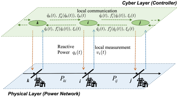
Fig. 6. Information flow of OPTDIST-VC.
