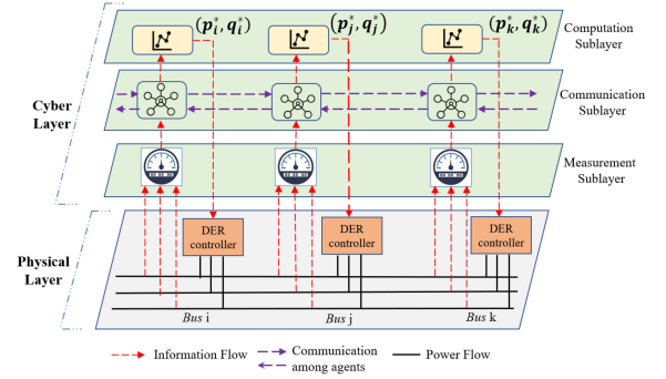
Fig. 9. An online distributed algorithm architecture.
