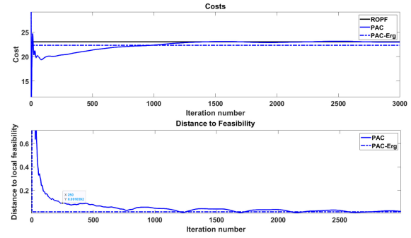
Fig. 8. Convergence characteristics for the PAC algorithm showing. (a) Costs comparison between centralized OPF and PAC. (b) Distance to feasibility.
