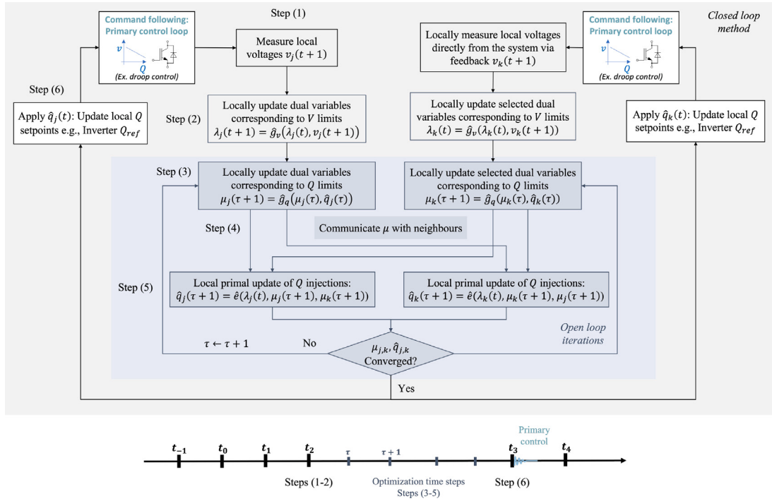
Fig. 5. Example workflow for a distributed optimization method with feedback-based methodology, based off of Bolognani et al. (2019) and Ortmann et al. (2020). Note that while the open-loop approach in Fig. 4 uses both P and Q injections as decision variables or actuation inputs, the feedback-based approach here only uses Q injections.
