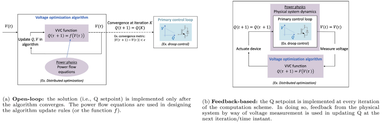
Fig. 3. Open-loop and feedback-based solution methodologies for voltage control.
