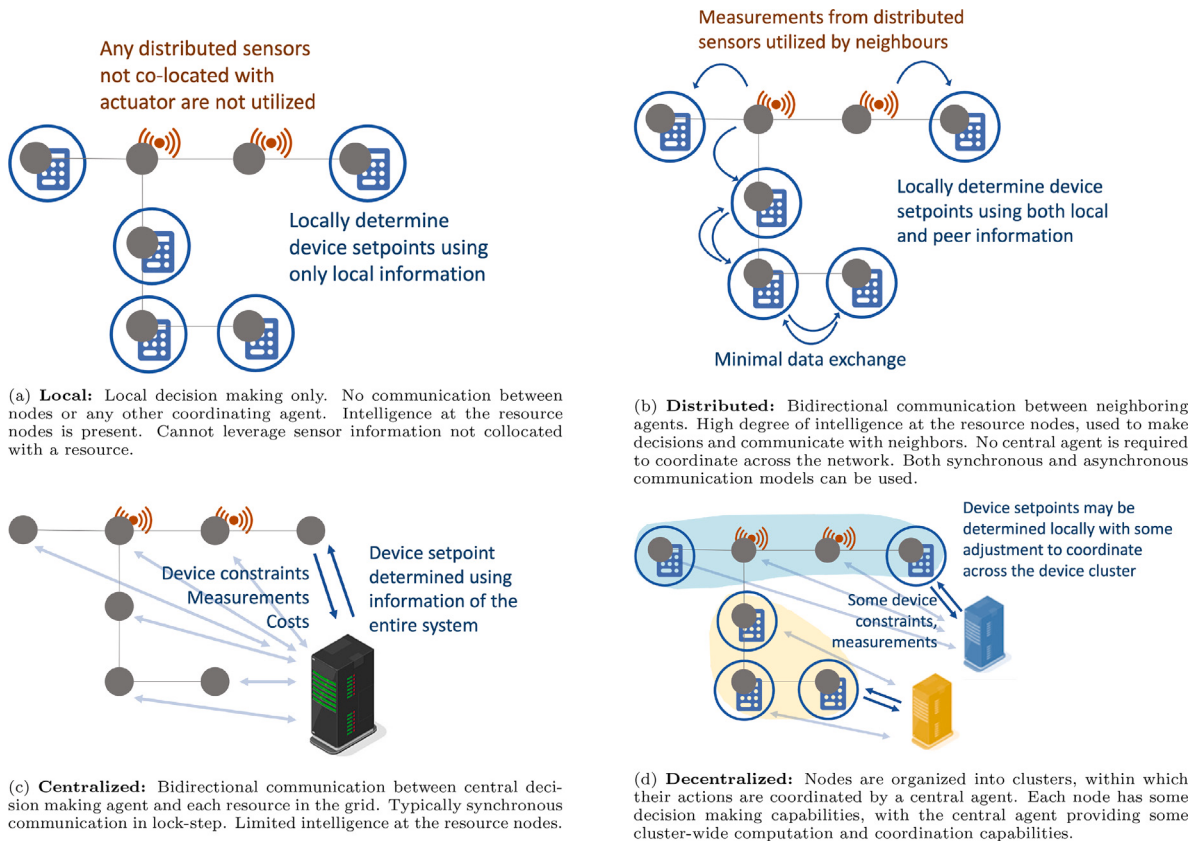
Fig. 2. Different types of coordination mechanisms used for voltage control.
