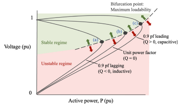
Fig. 1. Nose curves demonstrating the critical active power values for different values of the reactive power.
