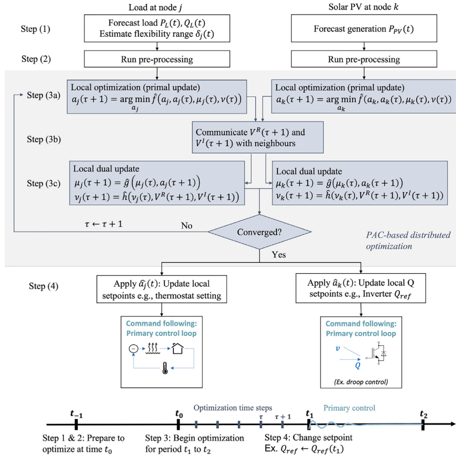
Fig. 4. Example workflow for an open-loop distributed optimization method, illustrating the Proximal Atomic Coordination algorithm from Haider and Annaswamy (2022) and Romvary et al. (2022).
