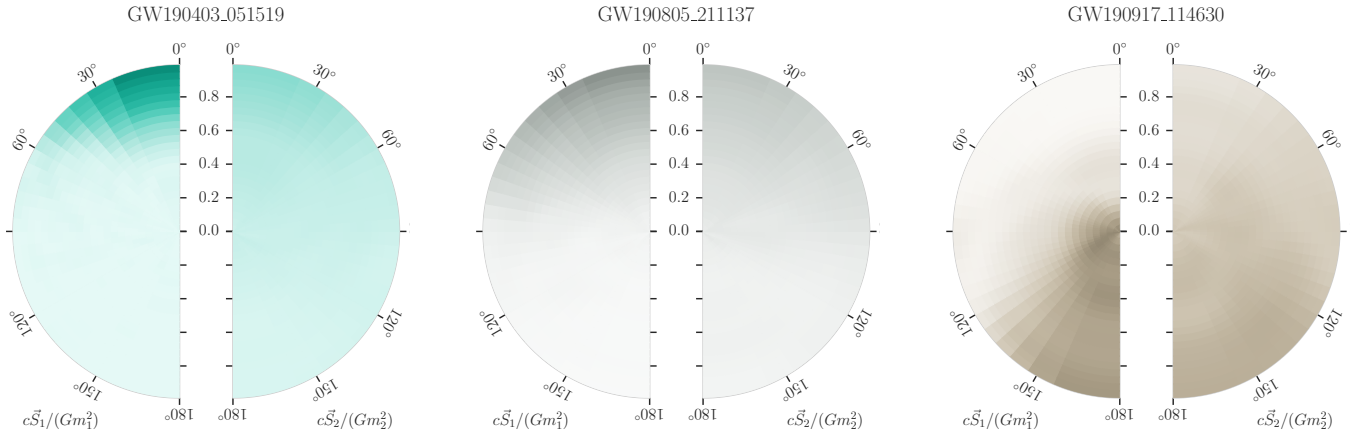
FIG. 6. The dimensionless spin parameters \tilde{\chi}_i = c\vec{S}_i/(Gm_i^2) estimated for individual binary components of selected sources. The radial distance of a given pixel on the left (right) of each disk, away from the center of the circle, corresponds to |\tilde{\chi}| for the more (less) massive compact object. Each pixel's angle from the vertical axis represents \theta_{\text{LS}} , the angle between the spin vector \vec{S} and the Newtonian orbital angular momentum. All pixels have equal prior probability with the shading denoting the relative posterior probability of the pixels, after marginalization over azimuthal angles. The events follow the same color scheme used in Fig. 3.
