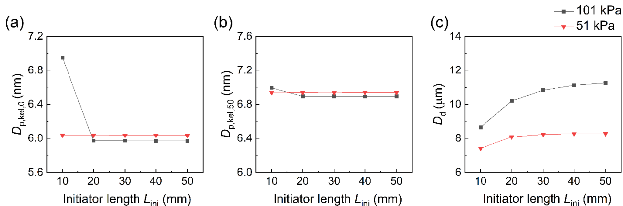
Figure 7. Effect of initiator length ( L_{ini} ) at 51 kPa and 101 kPa on (a) minimum activated size, D_{p,kei,0} , (b) 50% cut-off size, D_{p,kei,50} , and (c) final growth particle size at the outlet of the moderator along the centerline ( r = 0 ), D_d . The condensational growth of 8 nm particles was tested as seed particles.
