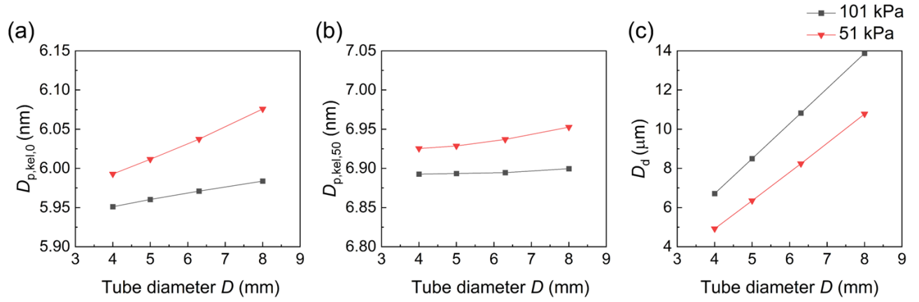
Figure 6. Effect of tube diameter ( D ) at 51 kPa and 101 kPa on (a) minimum activated size, D_{p,rel,0} , (b) 50% cut-off size, D_{p,rel,50} , and (c) final growth particle size at the outlet of the moderator along the centerline ( r = 0 ), D_d . The condensational growth of 8 nm particles was tested as seed particles.
