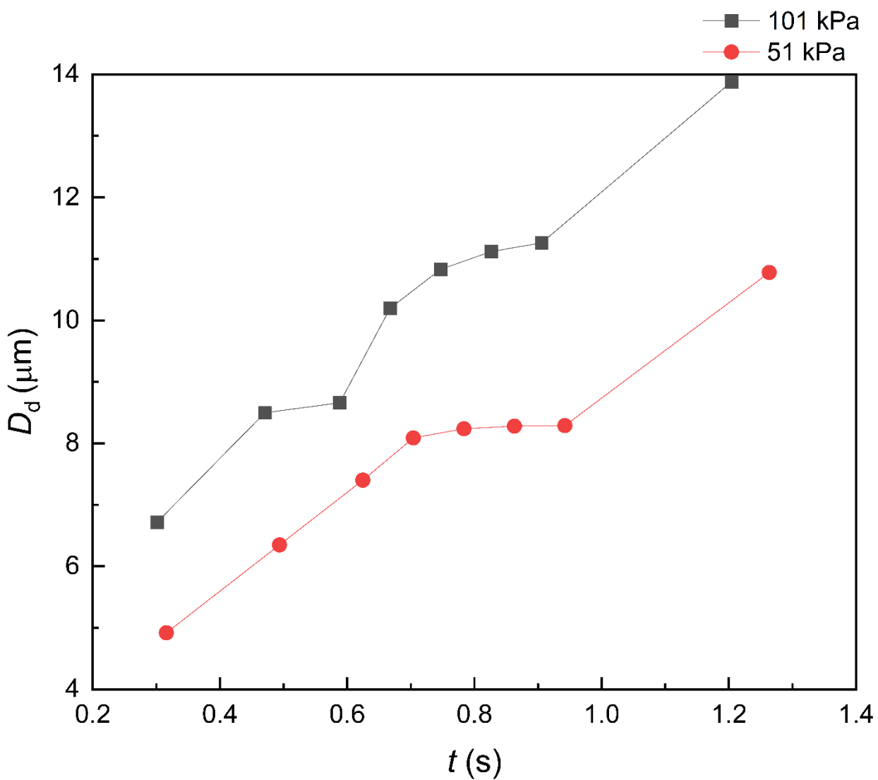
Figure S3. Effect of allowed particle growth time ( t ) at the standard pressure and the reduced pressure of 51 kPa on final growth particle size at the outlet of moderator along the centerline ( r = 0 ), D_d . The condensational growth of 8 nm particles was tested as seed particles.
