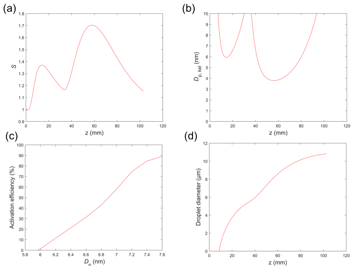
Figure S1. Evaluation of particle activation and droplet growth performance at the default temperature condition of T_{\text{con}} = 30 °C, T_{\text{ini}} = 59 °C, T_{\text{mod}} = 10 °C. (a) saturation ratio ( S ), (b) Kelvin equivalent size ( D_{p, \text{kel}} ) as a function of distance along the axis centerline ( r = 0 ) of the tube, (c) activation efficiency as a function of particle diameter, and (d) droplet growth size as a function of distance along the axis of the tube. The condensational growth of 8 nm particles was simulated along the centerline ( r = 0 ).
