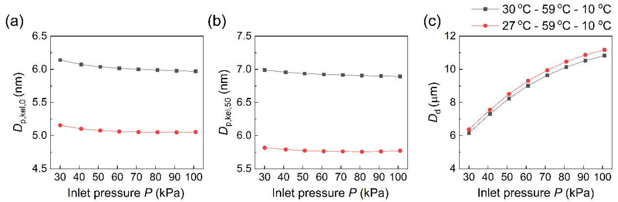
Figure 5. Effect of inlet operation pressure at T_{con} - T_{ini} - T_{mod} of 27-59-10 °C and 30-59-10 °C on (a) minimum activated size, D_{p,kel,0} , (b) 50% cut-off size, D_{p,kel,50} , and (c) final growth particle size at the outlet of the moderator along the centerline ( r = 0 ), D_d . The condensational growth of 8 nm particles was tested as seed particles.
