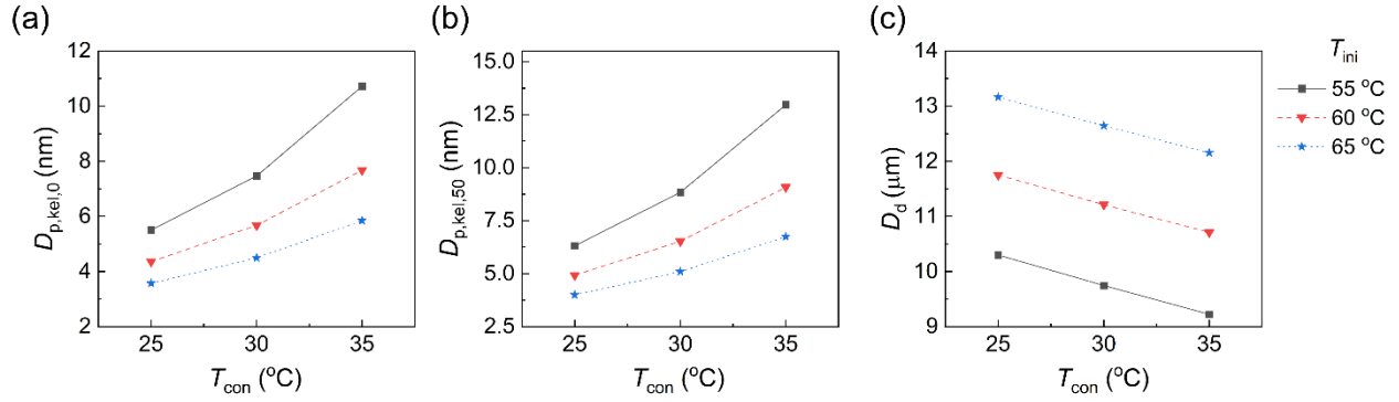
Figure 3. Effect of conditioner ( T_{con} ) and initiator temperature ( T_{ini} ) on (a) minimum activated size, D_{p,keI,0} , (b) 50% cut-off size, D_{p,keI,50} , and (c) final growth particle size at the outlet of the moderator along the centerline ( r = 0 ), D_d . The condensational growth of 15 nm particles was tested as seed particles.
