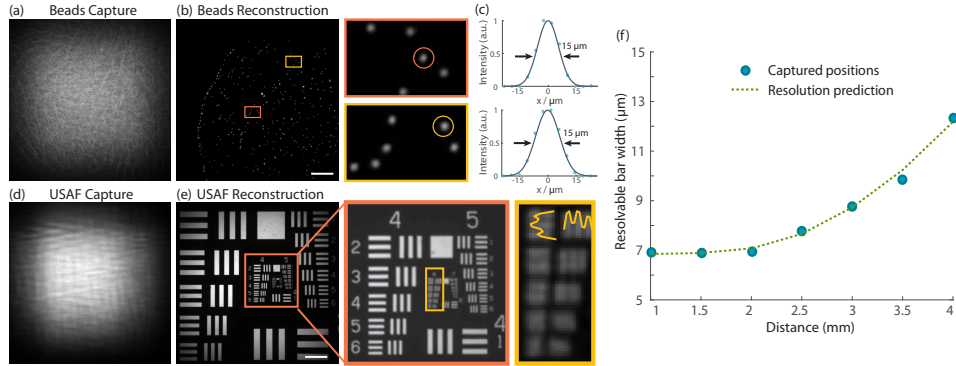
Fig. 3. System Characterization. (a) Experimental capture of 15\ \mu\text{m} green fluorescent beads spread on a glass slide. (b) The reconstruction of 15\ \mu\text{m} green fluorescent beads spread on a glass slide. Single beads are clearly visible in the small region zoom-ins. Scale bar, 500\ \mu\text{m} . (c) The lateral profile of two representatives reconstructed beads in the circle in panel b. (d) Experimental capture of a negative USAF target with an added fluorescent background. (e) The reconstruction of the negative USAF target. Zoom-in shows groups 4,5 and 6. Group 6 element 2 ( < 7\ \mu\text{m} features) can be resolved in the reconstructed image. Scale bar, 500\ \mu\text{m} . (f) Resolution evaluation at different imaging depths.
