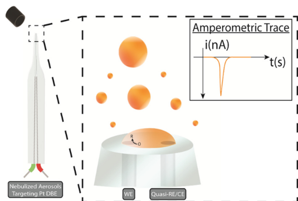
Fig. 1 Illustration of an aerosol spanning the distance between platinum disks and producing a transient of current from an electrochemical reaction, recorded via an amperometric i - t trace. The typical transient is on the order of a second.
