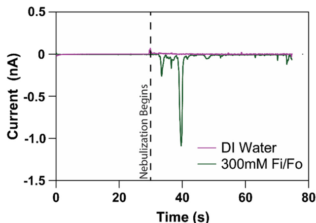
Fig. 3 Amperometric i - t trace showing discrete aerosol impact events, most notably at 33 and 40 s. The potential is held at +0.3 V for this experiment. When the solution of 300 mM hexacyanoferrate(II/III) (Fi/Fo) is nebulized (beginning at 30 s), the ferrocyanide in aerosols that impact the dual-barrel electrode will convert to ferricyanide, producing a spike in current. The distance from the nebulizer to the electrode tip was held at \sim 2.5 cm.
