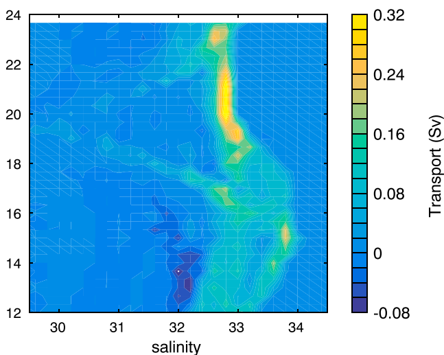
Figure 10. The transport across the 100-m isobath, between the model western boundary and x = 1,000 km as a function of salinity (0.2-ppt increments) and time. This is calculated over the second year of integration only. The 100-m isobath is indicated in Figure 3 by the bold green line.
