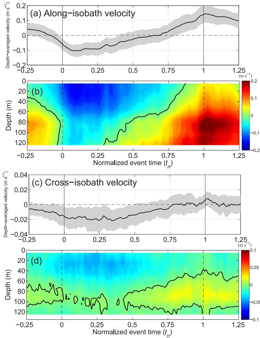
Fig. 5. Composite upwelling event constructed from the 115 individual events. (a) Depth-averaged along-isobath velocity (positive is eastward). The shading represents the standard error. (b) Depth-dependent along-isobath velocity. (c) Depth-averaged cross-isobath velocity (positive is offshore). (d) Depth-dependent cross-isobath velocity. The 0 contours are highlighted. The units are m s^{-1} .
