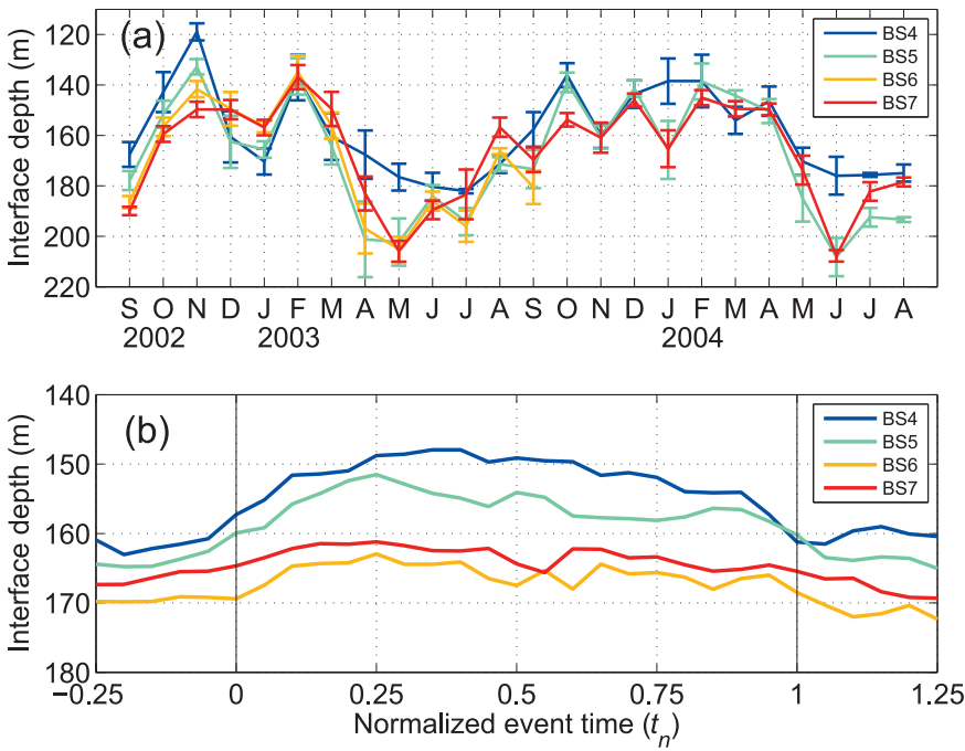
Fig. 11. (a) Time series of monthly-averaged PW-AW interface depth for the four offshore SBI moorings (2002–2004). The standard errors are indicated. (b) Interface depth for the composite upwelling event constructed using the SBI data, for each of the four moorings.
