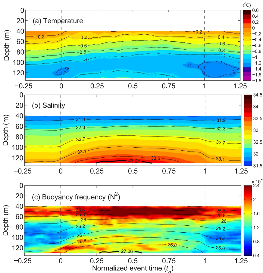
Fig. 4. Composite upwelling event constructed from the 115 individual events. (a) Potential temperature ( ^\circ\text{C} ), (b) salinity, and (c) buoyancy frequency (color, \text{N}^2 \text{ s}^{-2} ) overlain by potential density (contours, \text{kg m}^{-3} ). The PW-AW interface is denoted by thick lines.
