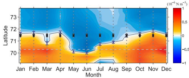
Fig. 14. Latitude-time distribution of the climatological monthly mean wind stress curl ( \times 10^{-6} \text{ N m}^{-3} ) close to 152^\circ\text{W} for the time period 2000–2013. The zero-curl contour with standard error (blue bars) is highlighted. The grey dashed line marks the location of coastline, and the grey dots are ASR data points. Black dots denote the mooring locations. (For interpretation of the references to color in this figure legend, the reader is referred to the web version of this article.)
