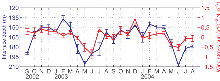
Fig. 13. Time series of monthly-averaged PW-AW interface depth (m, blue) and monthly area-averaged wind stress curl ( \times 10^{-6} \text{ N m}^{-3} , red) for September 2002 – August 2004. The standard errors are included. (For interpretation of the references to color in this figure legend, the reader is referred to the web version of this article.)
