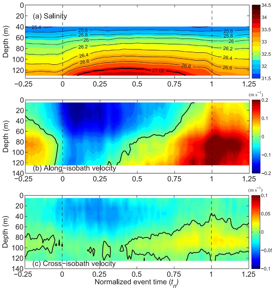
Fig. 8. Composite upwelling event constructed from the 85 individual AW-type upwelling events from 2002 to 2004. (a) Salinity (color) overlaid by potential density (contours, \text{kg m}^{-3} ). The thick lines indicate the PW-AW interface. (b) Along-isobath velocity (positive is eastward). (c) Cross-isobath velocity (positive is offshore). The 0 contours are highlighted.
