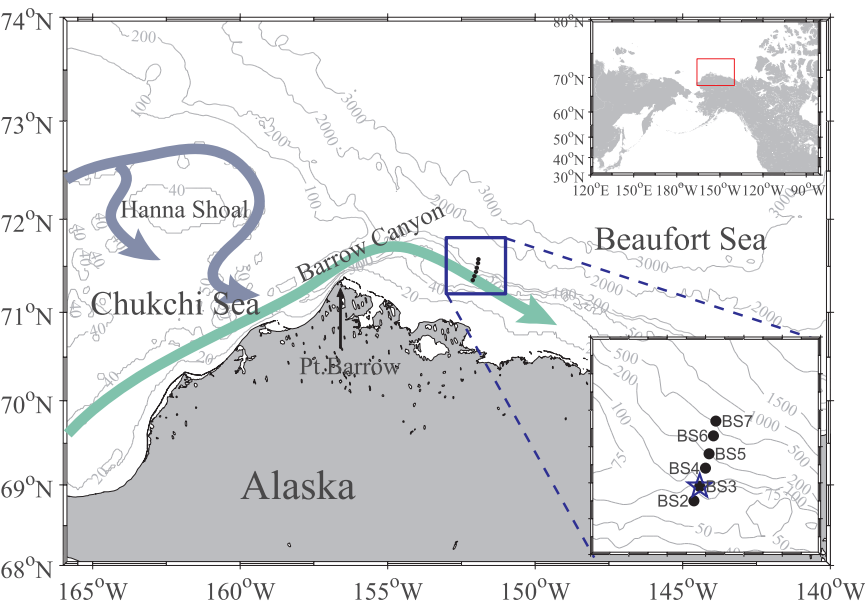
Fig. 1. Locations of the moorings (black circles) used in the study and the schematic circulation of the region. Mooring BS3 (blue star) was deployed for 6 years, the others deployed for 2 years. The green arrow denotes the Alaskan Coastal Current and Beaufort shelfbreak jet. The blue arrows are the schematic Pacific Water pathways on the northeast Chukchi shelf. The meteorological data used in the study came from the weather station at Barrow, AK. The bathymetric contours are in meters. (For interpretation of the references to color in this figure legend, the reader is referred to the web version of this article.)
