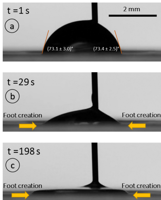
Fig. 2 A hydrogel substrate swells after being in contact with a water droplet, forming a foot. Here, we show (a) the droplet one second after contact, (b) the start of foot creation as water is diffused into the gel after 29 s, and (c) a more visible foot after 198 s. Note that in panels b and c, the droplet has been intentionally recessed to show foot creation.
