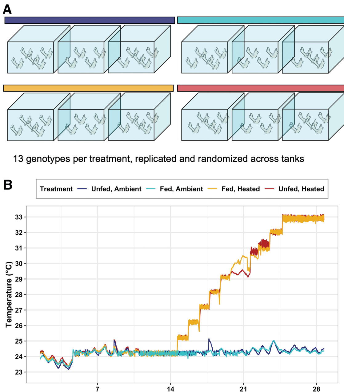
Fig. 1. (A) Experimental design showing tank setup and coral distributions across tanks and experimental treatments. Each treatment had three replicate tanks, with a common temperature controller and sump. Lighting regimes were identical across tanks. (B) Temperatures of experimental treatments throughout the 28-d experiment. P indicates when F/F_m measurements were taken and the asterisk indicates when corals were flash frozen for phenotypic and gene expression analyses.
